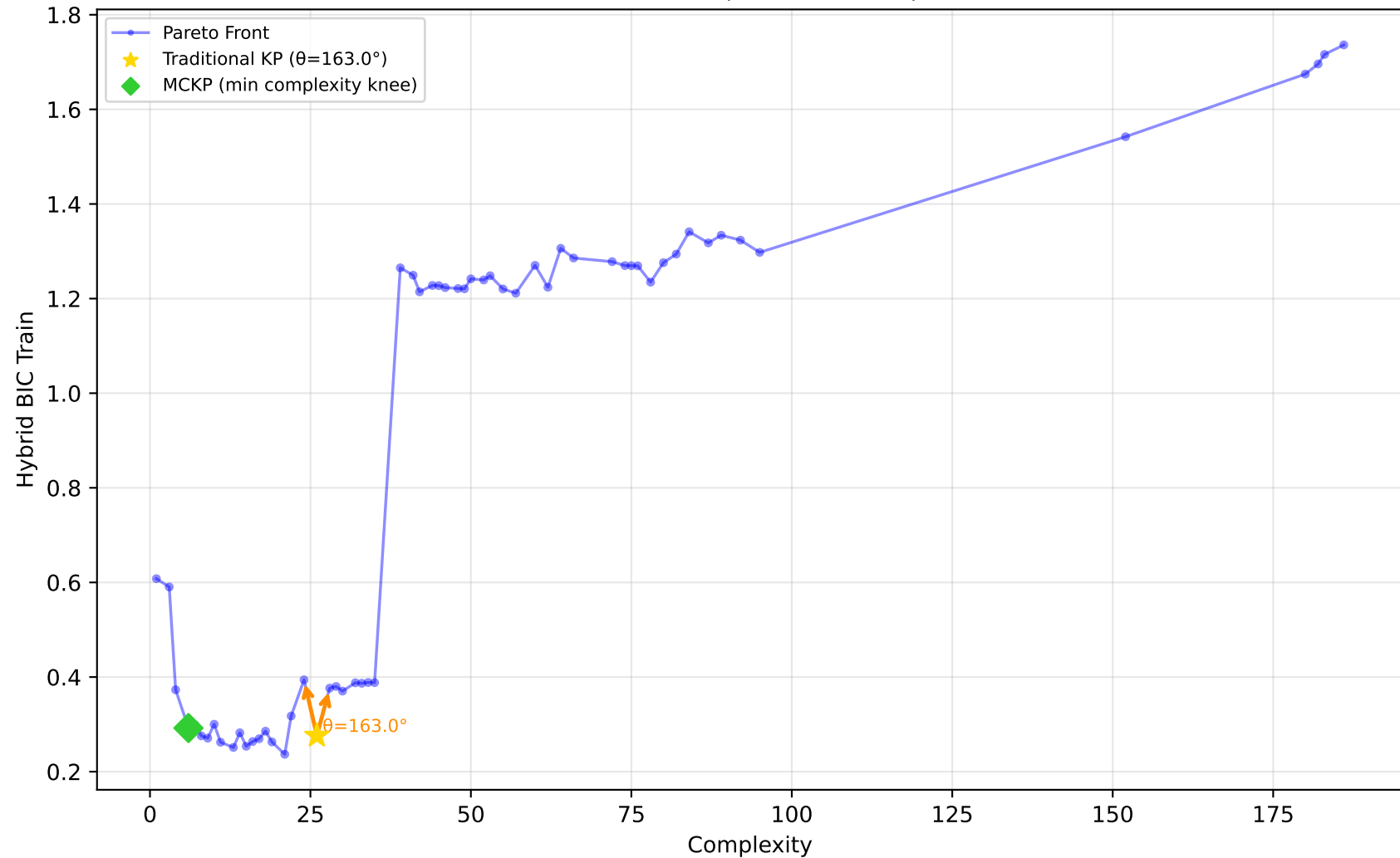
228_elusage - Run 26 - MVP - Hybrid BIC Train \lambda_1=0.00, \lambda_2=0.00, \lambda_3=1.00 | Difficulty: 0.44 | Method: mckp
