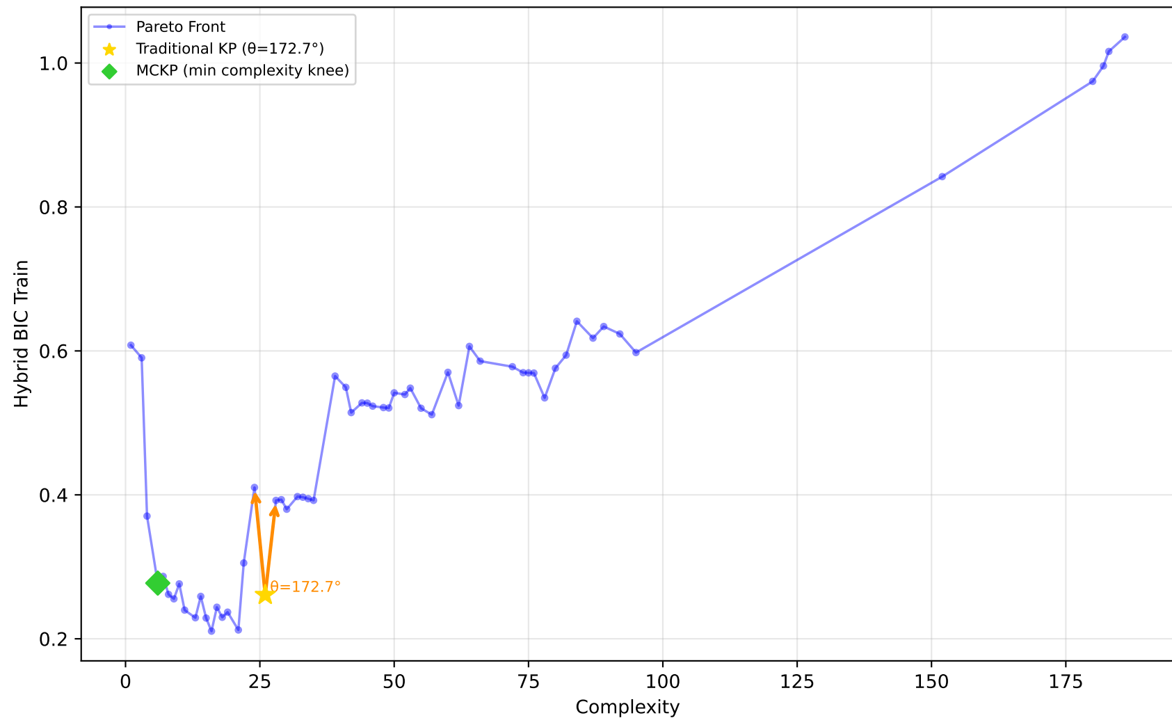
228_elusage - Run 26 - MVP - Hybrid BIC Train \lambda_1=0.00, \lambda_2=0.30, \lambda_3=0.00 | Difficulty: 0.44 | Method: mckp
