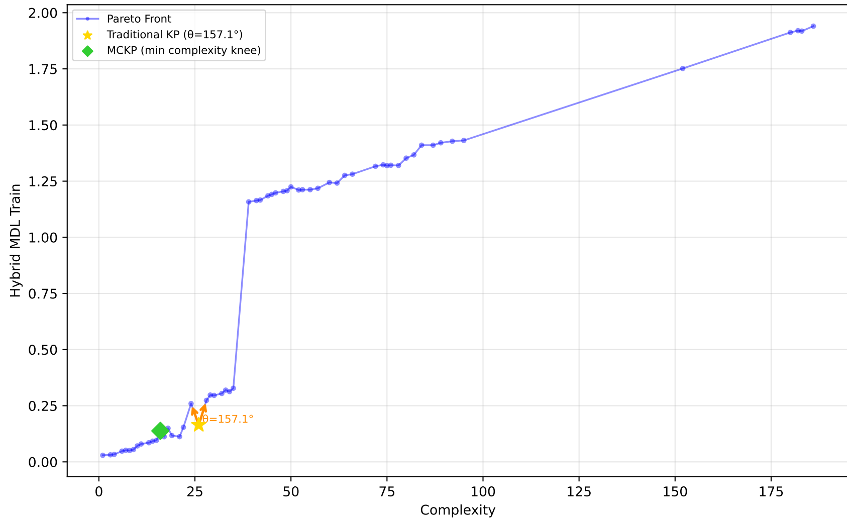
228_elusage - Run 26 - MVP - Hybrid MDL Train \lambda_1=0.00, \lambda_2=0.00, \lambda_3=1.00 | Difficulty: 0.44 | Method: mckp
