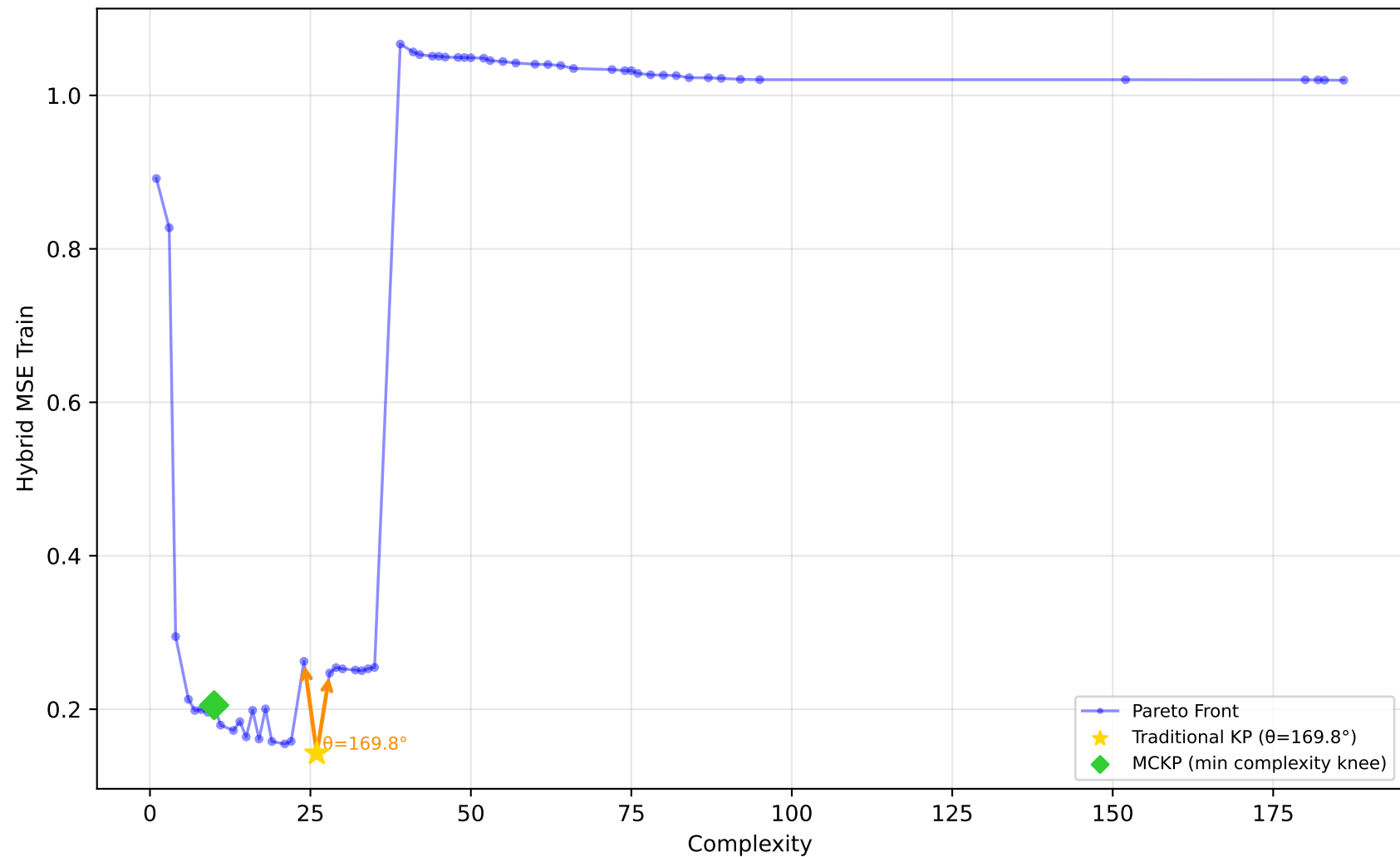
228_elusage - Run 26 - MVP - Hybrid MSE Train \lambda_1=0.00, \lambda_2=0.00, \lambda_3=1.00 | Difficulty: 0.44 | Method: mckp
