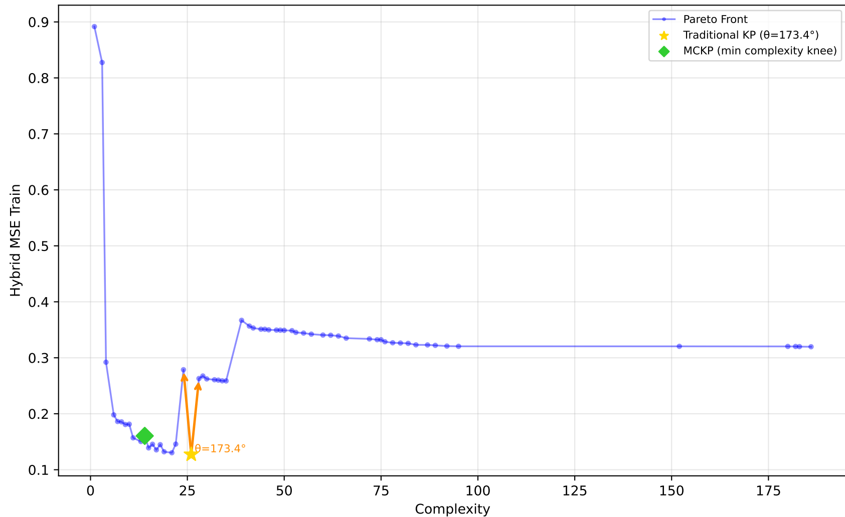
228_elusage - Run 26 - MVP - Hybrid MSE Train \lambda_1=0.00, \lambda_2=0.30, \lambda_3=0.00 | Difficulty: 0.44 | Method: mckp
