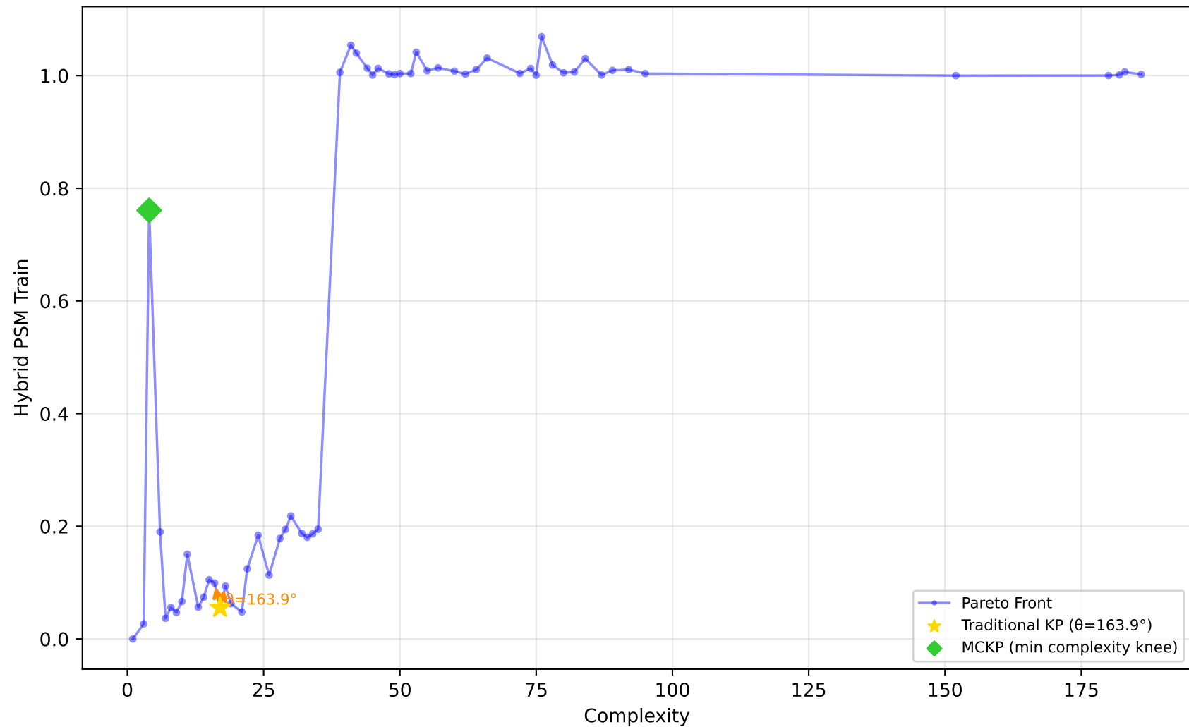
228_elusage - Run 26 - MVP - Hybrid PSM Train \lambda_1=0.00, \lambda_2=0.00, \lambda_3=1.00 | Difficulty: 0.44 | Method: mckp
