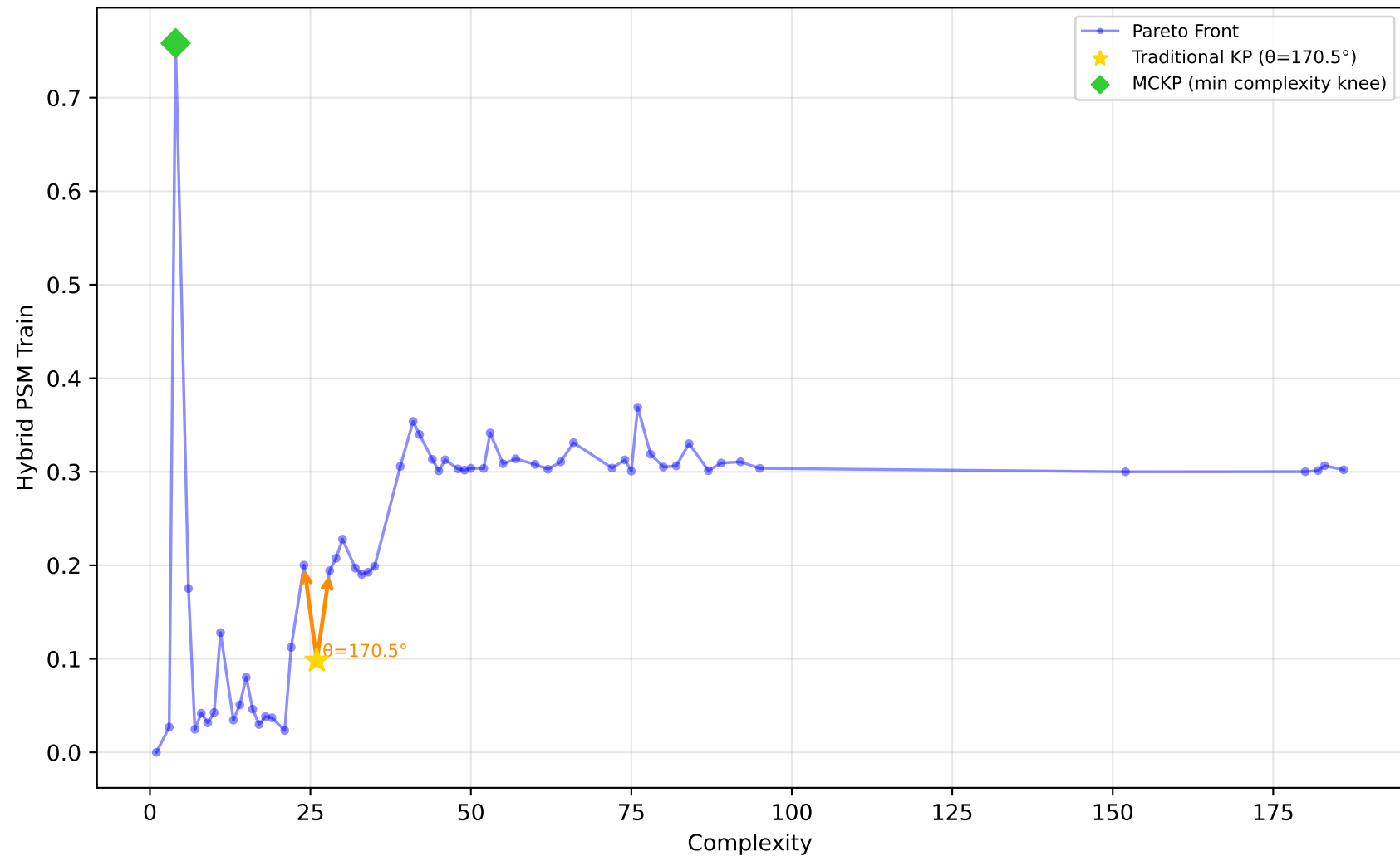
228_elusage - Run 26 - MVP - Hybrid PSM Train \lambda_1=0.00, \lambda_2=0.30, \lambda_3=0.00 | Difficulty: 0.44 | Method: mckp
