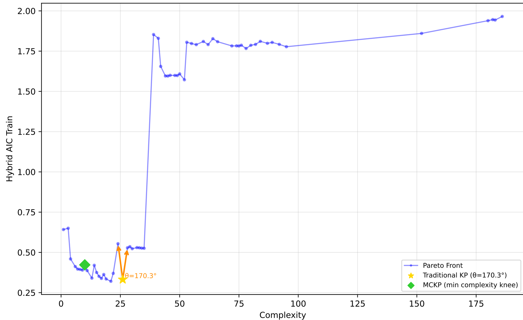
228_elusage - Run 26 - SVP - Hybrid AIC Train \lambda_1=0.60, \lambda_2=0.60, \lambda_3=1.00 | Difficulty: 0.44 | Method: mckp
