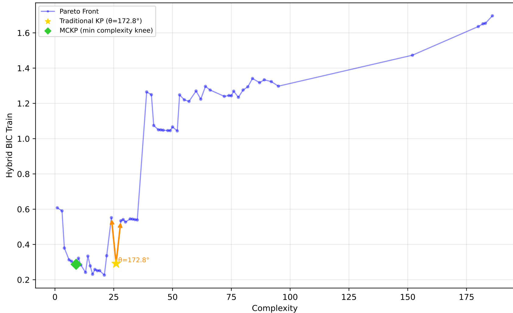
228_elusage - Run 26 - SVP - Hybrid BIC Train \lambda_1=0.00, \lambda_2=1.00, \lambda_3=0.00 | Difficulty: 0.44 | Method: mckp
