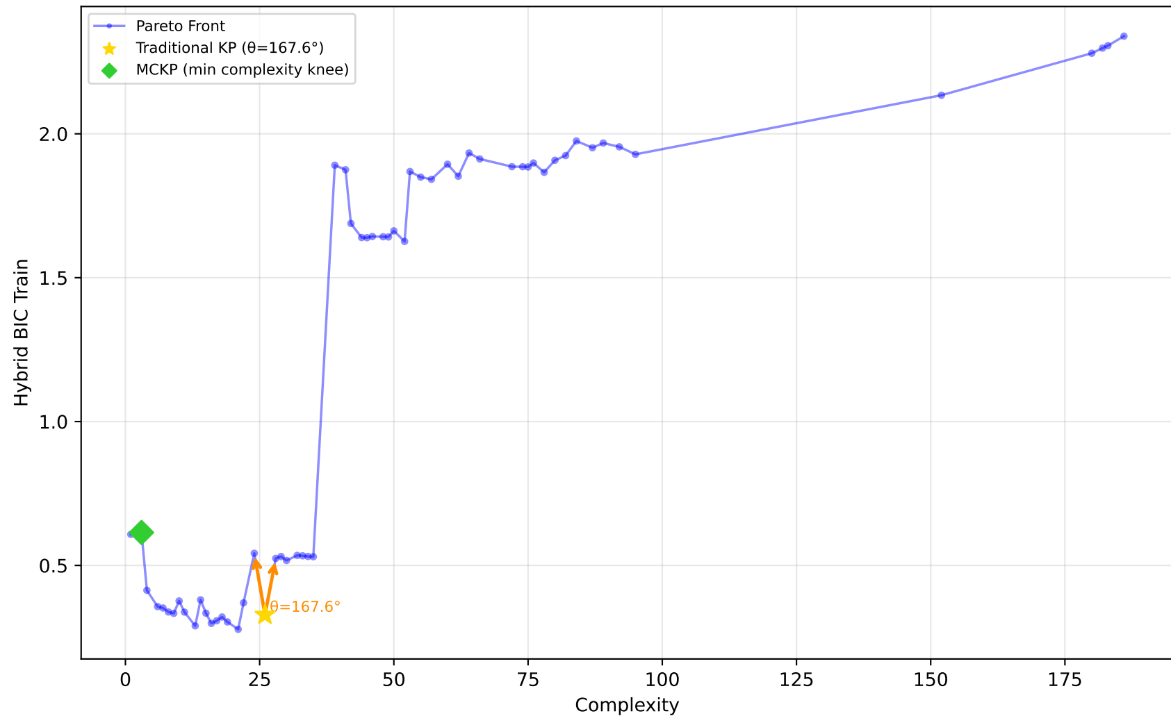
228_elusage - Run 26 - SVP - Hybrid BIC Train \lambda_1=0.60, \lambda_2=0.60, \lambda_3=1.00 | Difficulty: 0.44 | Method: mckp
