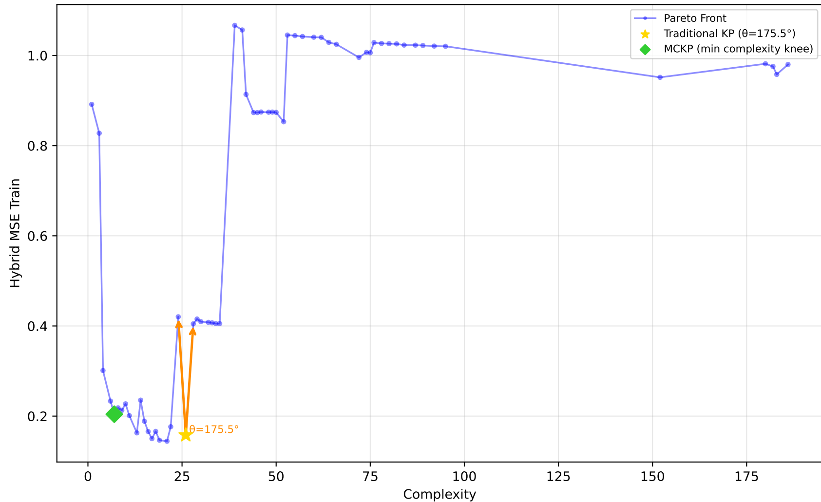
228_elusage - Run 26 - SVP - Hybrid MSE Train \lambda_1=0.00, \lambda_2=1.00, \lambda_3=0.00 | Difficulty: 0.44 | Method: mckp
