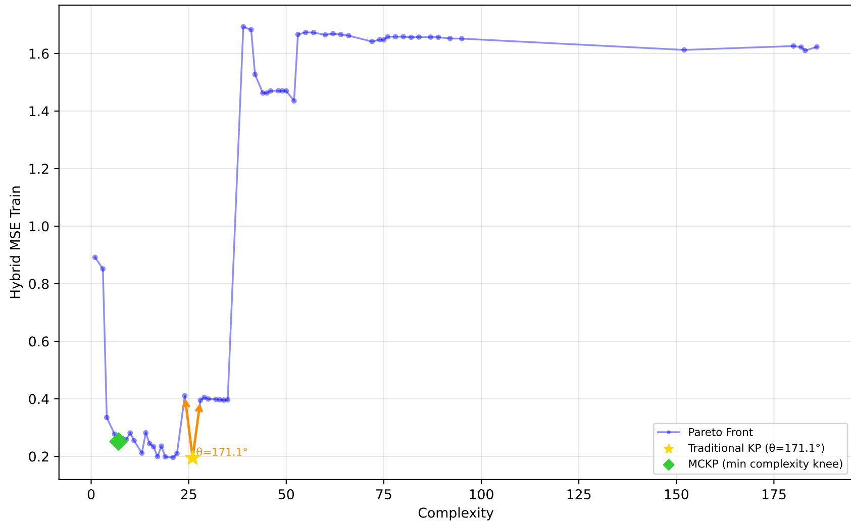
228_elusage - Run 26 - SVP - Hybrid MSE Train \lambda_1=0.60, \lambda_2=0.60, \lambda_3=1.00 | Difficulty: 0.44 | Method: mckp
