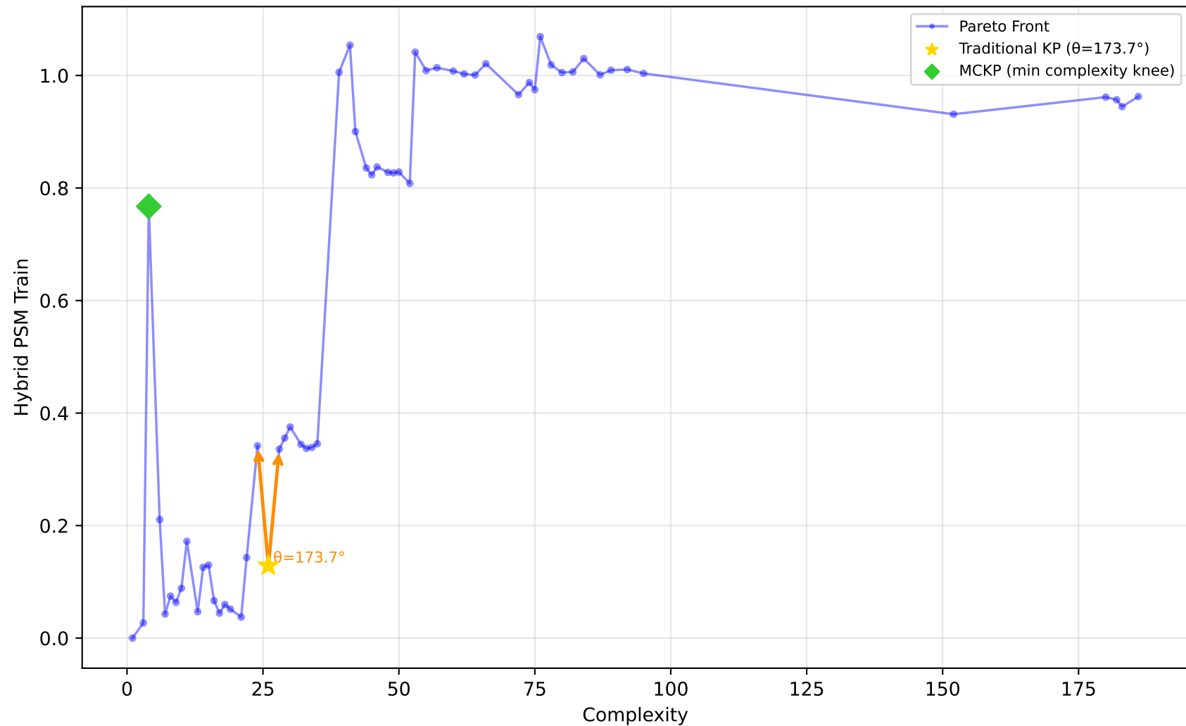
228_elusage - Run 26 - SVP - Hybrid PSM Train \lambda_1=0.00, \lambda_2=1.00, \lambda_3=0.00 | Difficulty: 0.44 | Method: mckp
