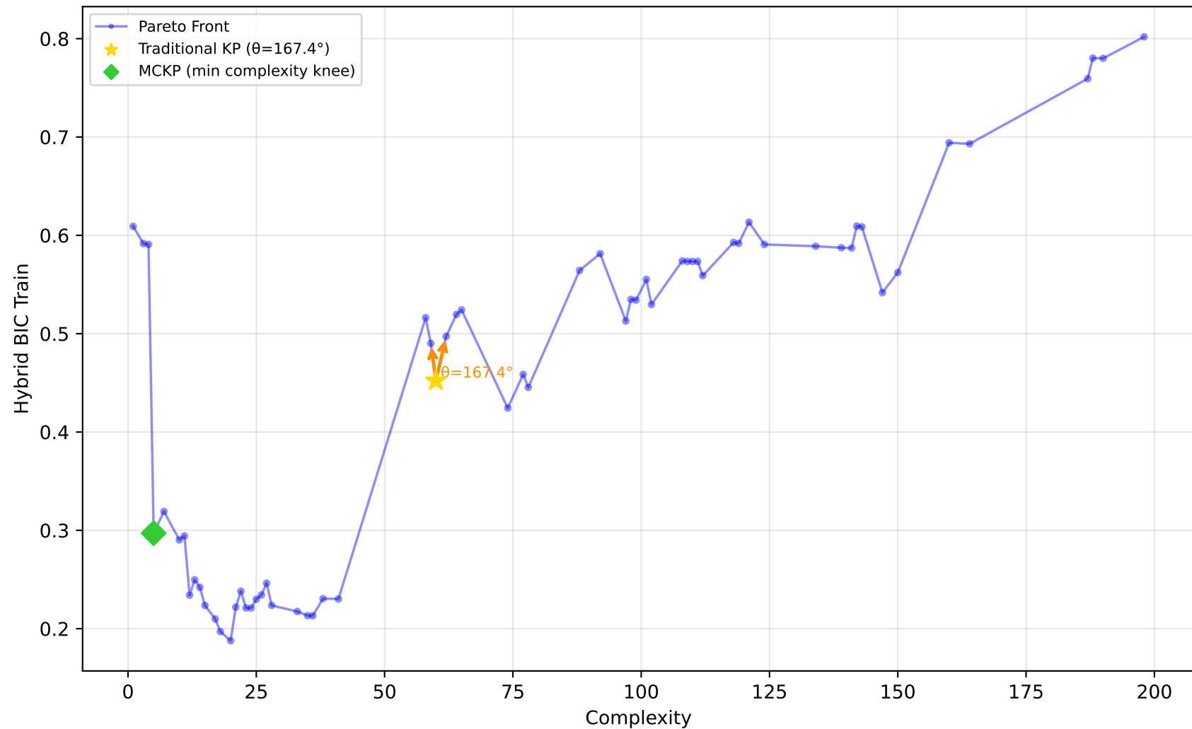
228_elusage - Run 27 - MVP - Hybrid BIC Train \lambda_1=0.00, \lambda_2=0.30, \lambda_3=0.00 | Difficulty: 0.83 | Method: hmr
