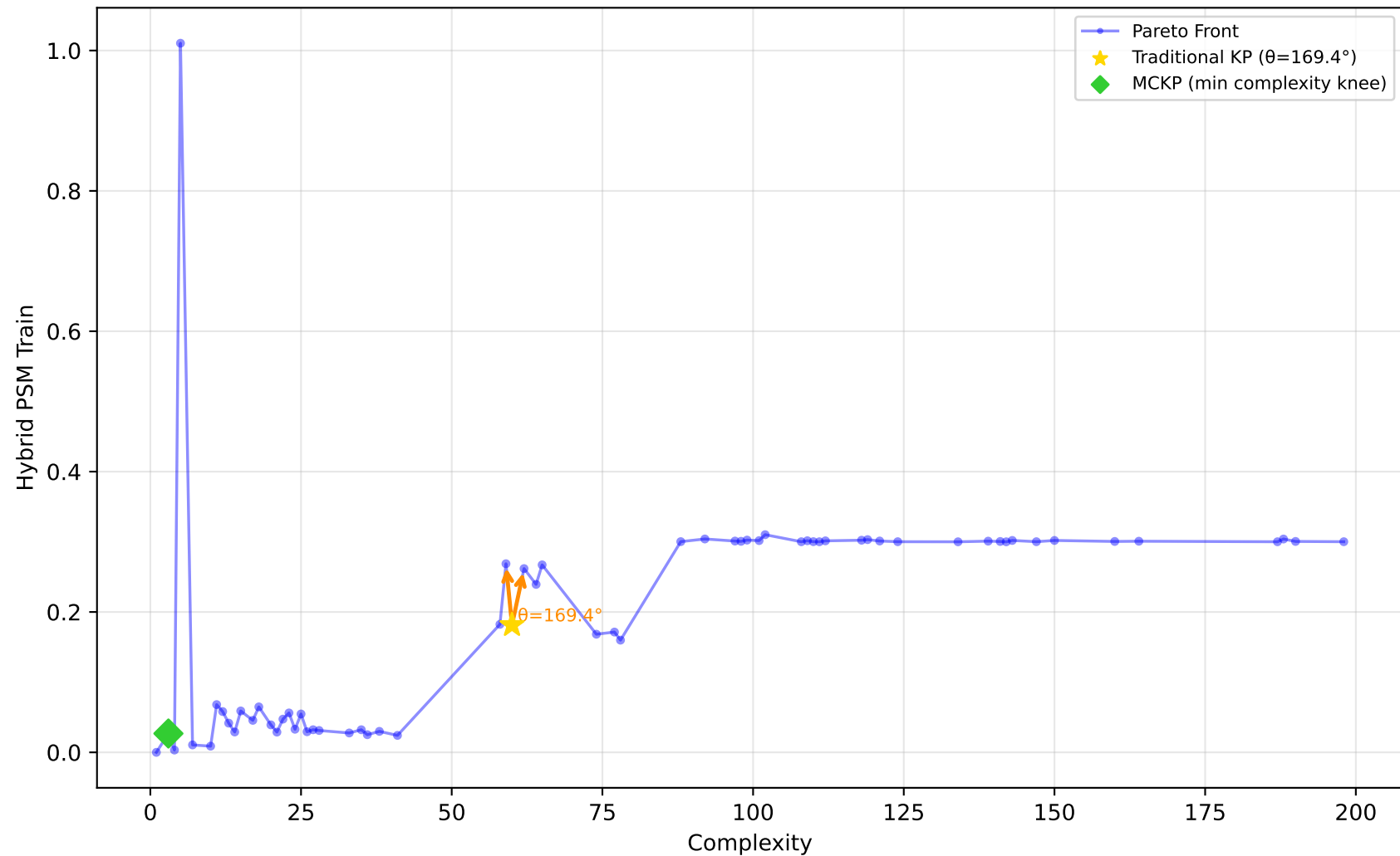
228_elusage - Run 27 - MVP - Hybrid PSM Train \lambda_1=0.00, \bar{\lambda}_2=0.30, \lambda_3=0.00 | Difficulty: 0.83 | Method: hmr
