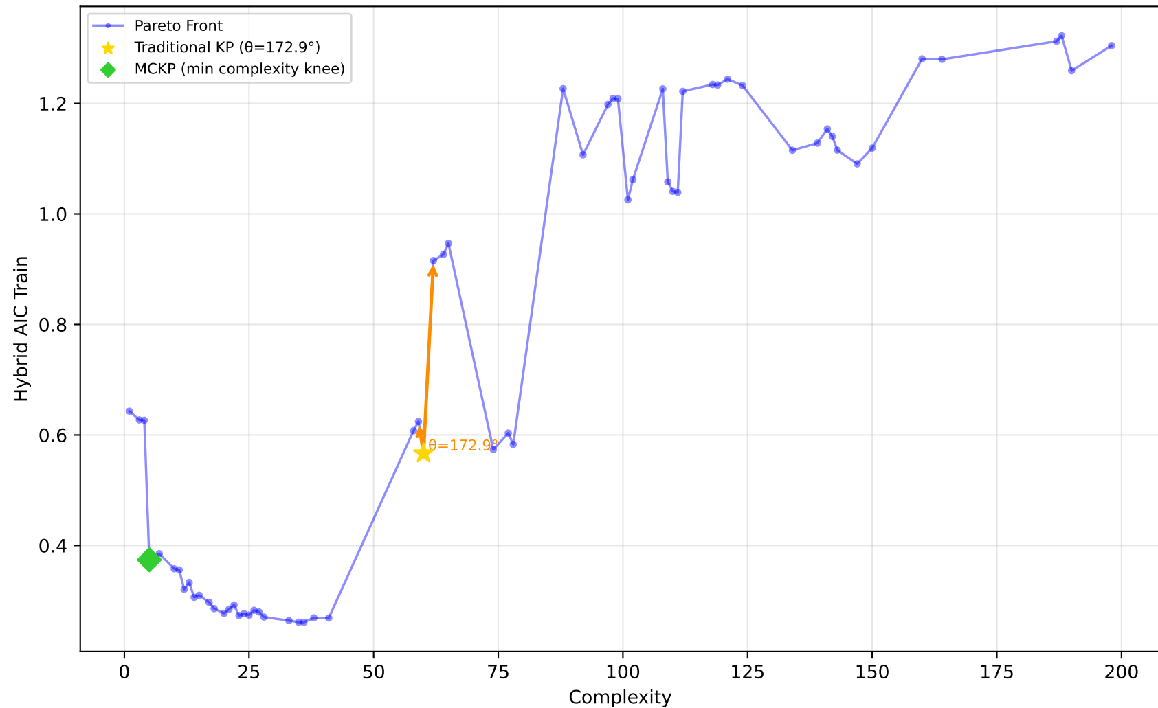
228_elusage - Run 27 - SVP - Hybrid AIC Train \lambda_1=0.00, \lambda_2=1.00, \lambda_3=0.00 | Difficulty: 0.83 | Method: hmr
