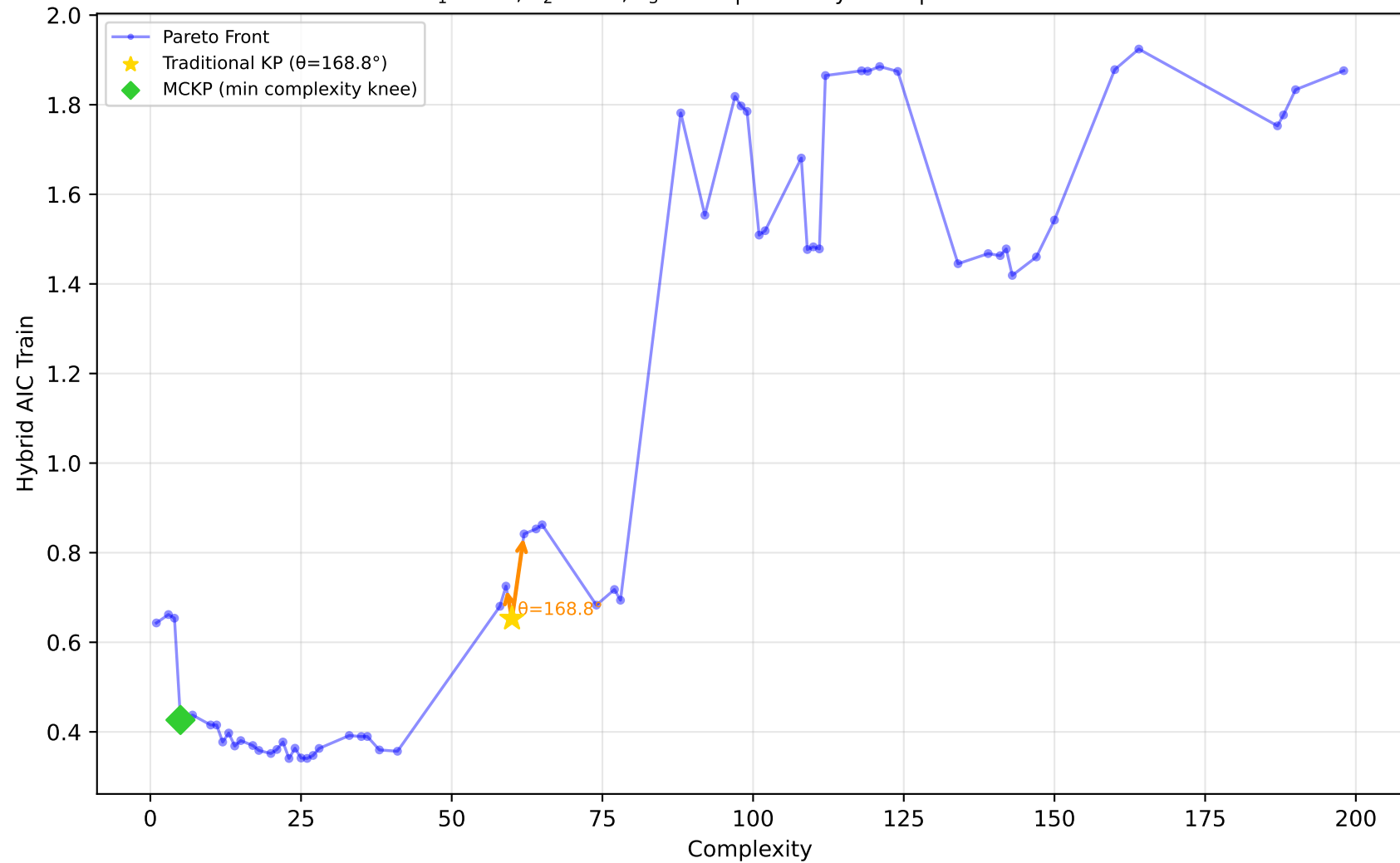
228_elusage - Run 27 - SVP - Hybrid AIC Train \lambda_1=0.60, \lambda_2=0.60, \lambda_3=1.00 | Difficulty: 0.83 | Method: hmr
