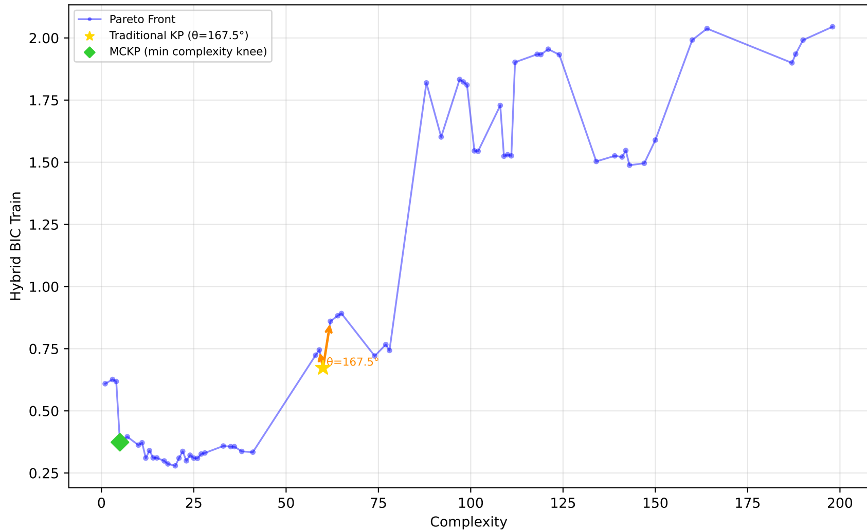
228_elusage - Run 27 - SVP - Hybrid BIC Train \lambda_1=0.60, \lambda_2=0.60, \lambda_3=1.00 | Difficulty: 0.83 | Method: hmr
