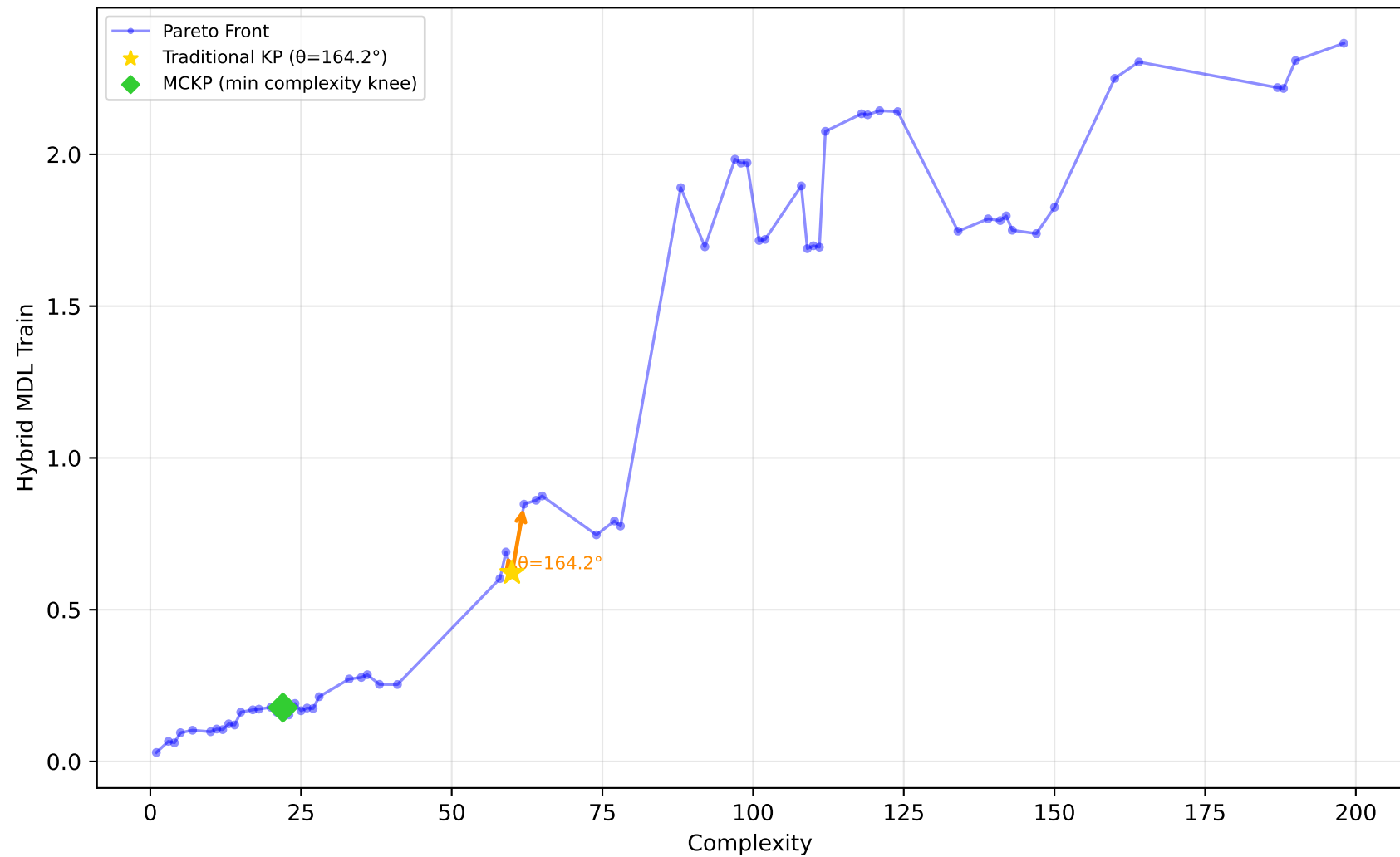
228_elusage - Run 27 - SVP - Hybrid MDL Train \lambda_1=0.60, \bar{\lambda}_2=0.60, \lambda_3=1.00 | Difficulty: 0.83 | Method: hmr
