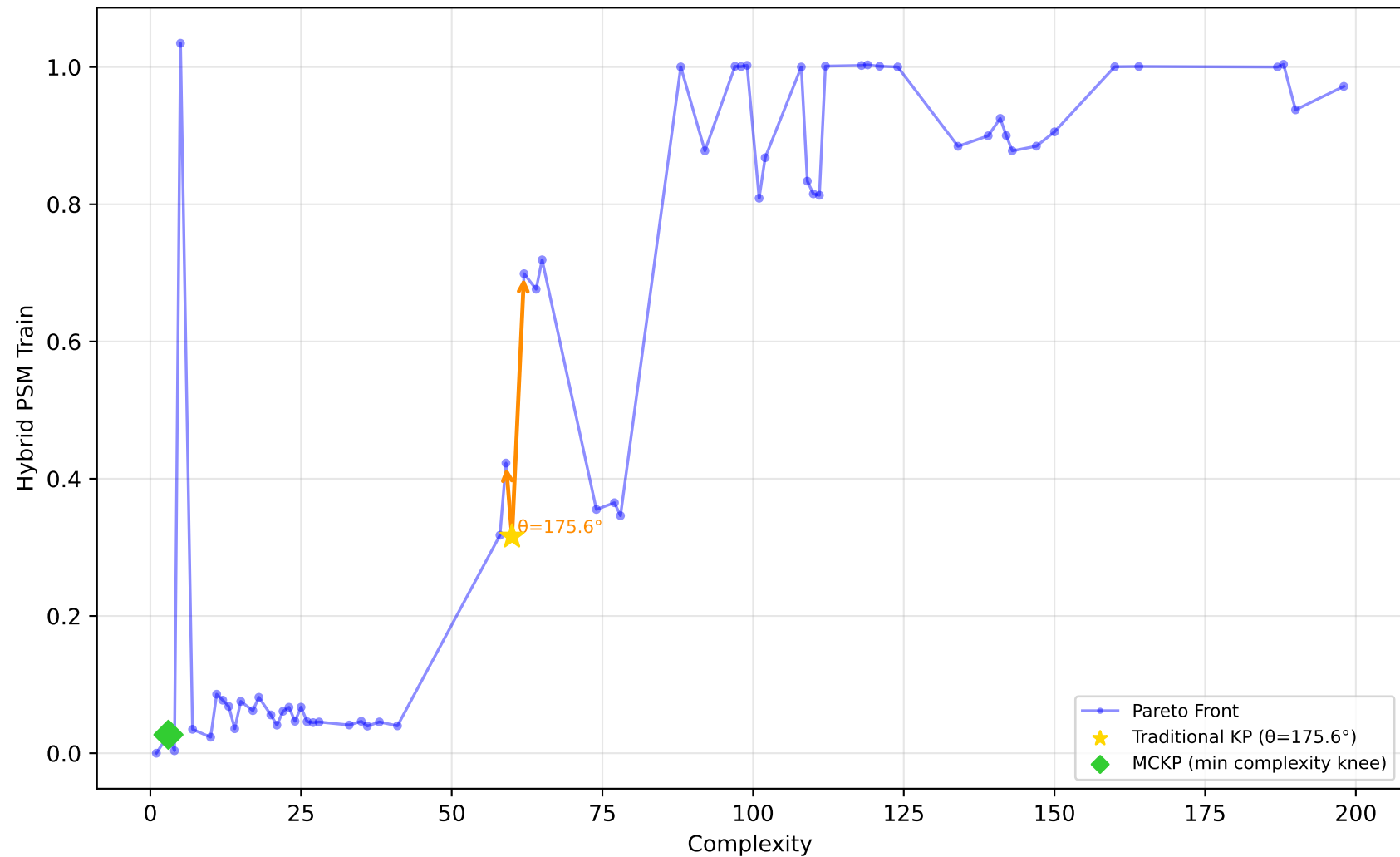
228_elusage - Run 27 - SVP - Hybrid PSM Train \lambda_1=0.00, \lambda_2=1.00, \lambda_3=0.00 | Difficulty: 0.83 | Method: hmr
