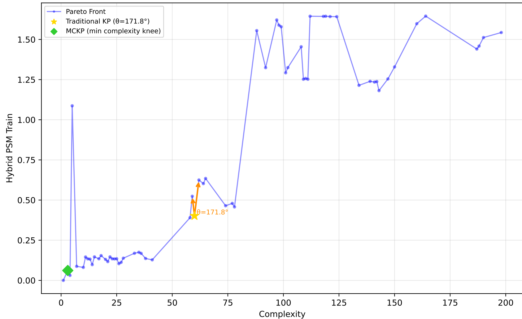
228_elusage - Run 27 - SVP - Hybrid PSM Train \lambda_1=0.60, \bar{\lambda}_2=0.60, \lambda_3=1.00 | Difficulty: 0.83 | Method: hmr
