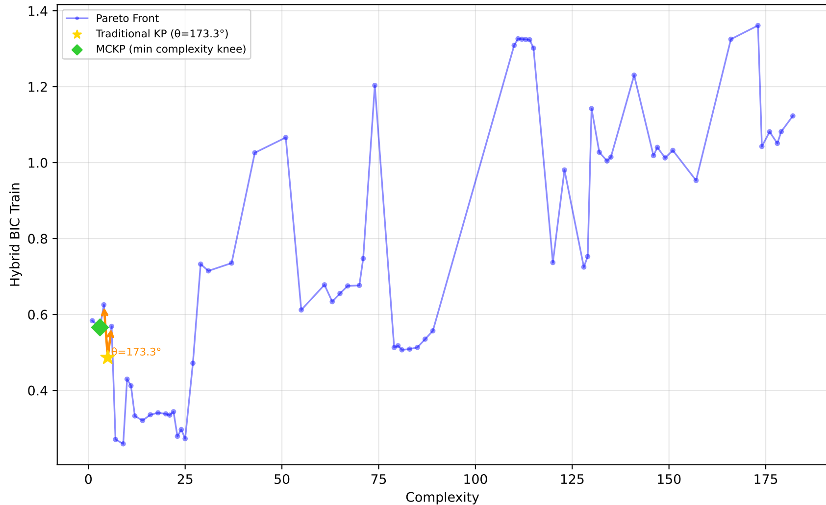
228_elusage - Run 28 - MVP - Hybrid BIC Train \lambda_1=0.00, \lambda_2=0.00, \lambda_3=1.00 | Difficulty: 0.53 | Method: mckp
