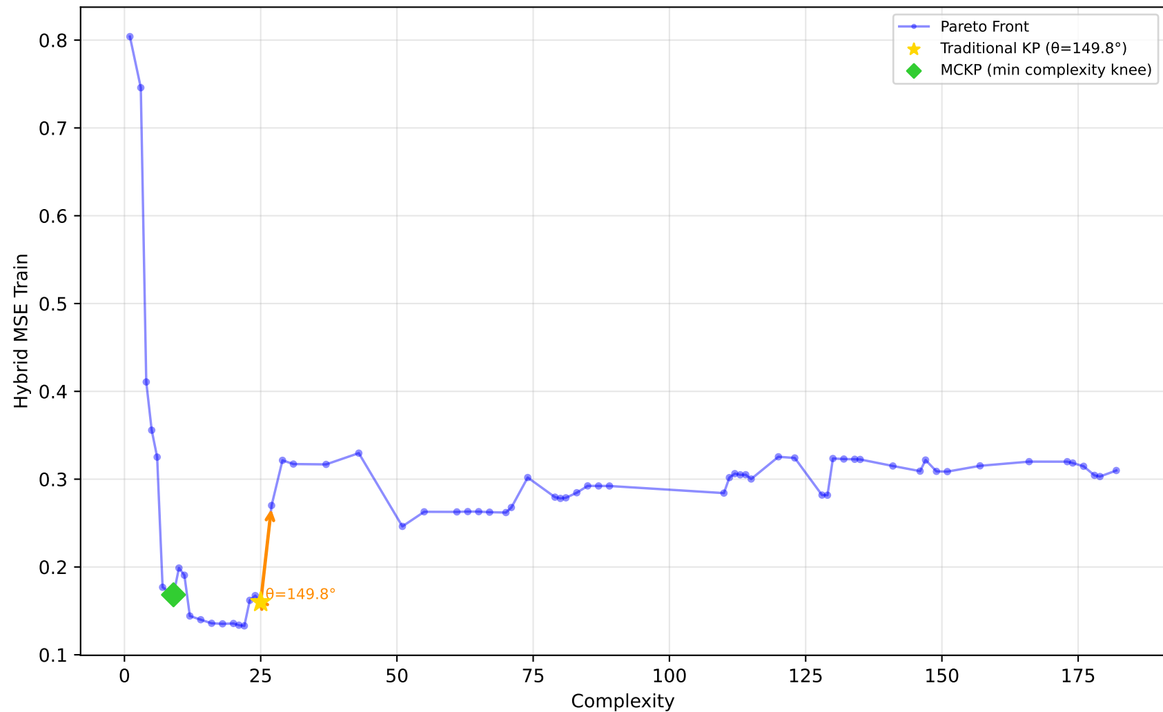
228_elusage - Run 28 - MVP - Hybrid MSE Train \lambda_1=0.00, \lambda_2=0.30, \lambda_3=0.00 | Difficulty: 0.53 | Method: mckp
