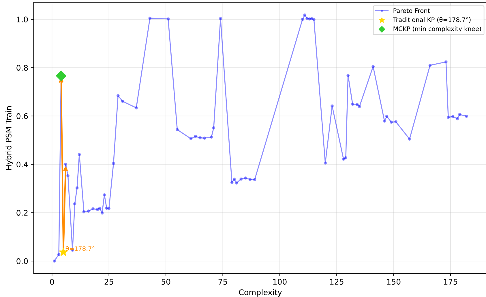
228_elusage - Run 28 - MVP - Hybrid PSM Train \lambda_1=0.00, \lambda_2=0.00, \lambda_3=1.00 | Difficulty: 0.53 | Method: mckp
