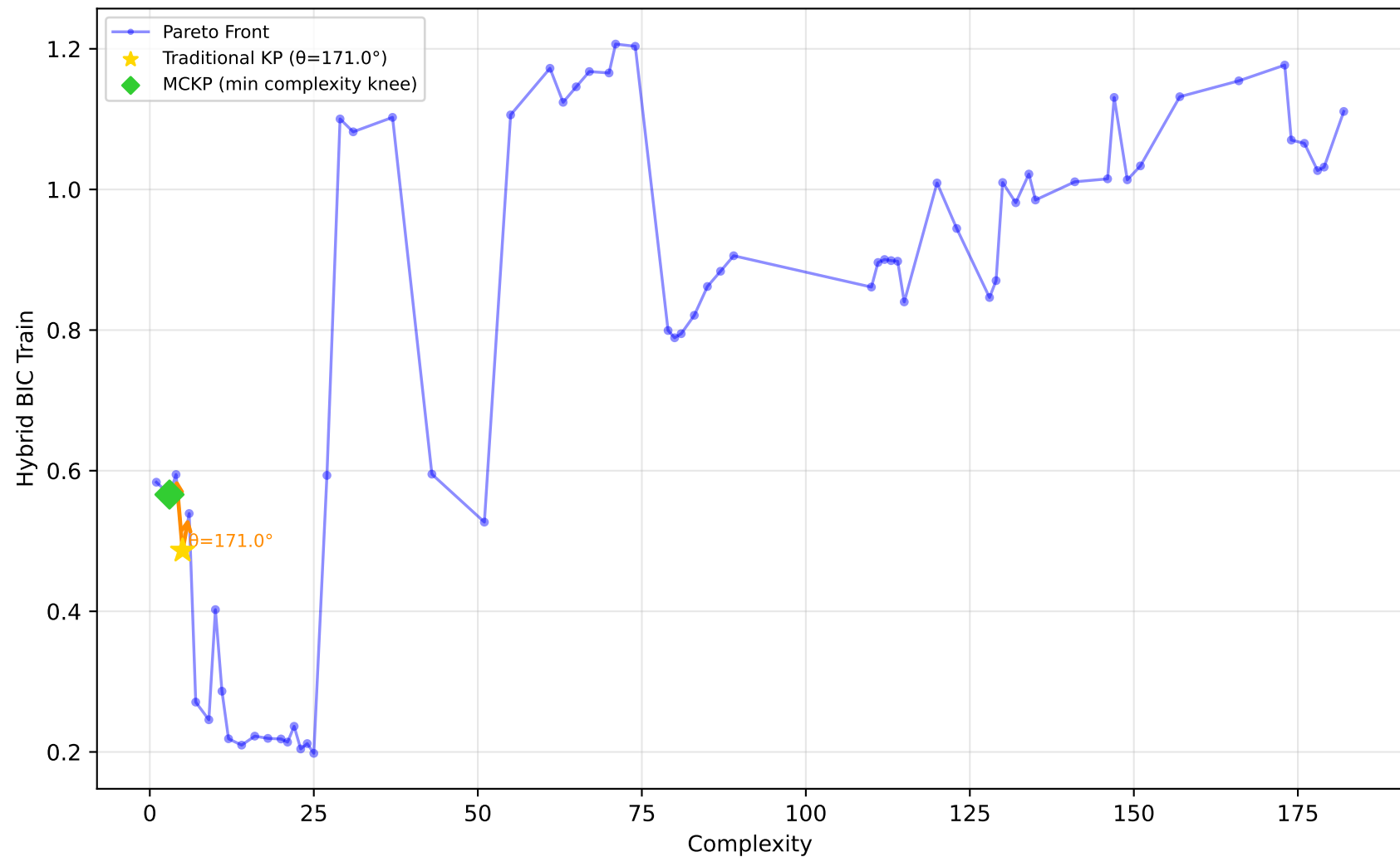
228_elusage - Run 28 - SVP - Hybrid BIC Train \lambda_1=0.00, \lambda_2=1.00, \lambda_3=0.00 | Difficulty: 0.53 | Method: mckp
