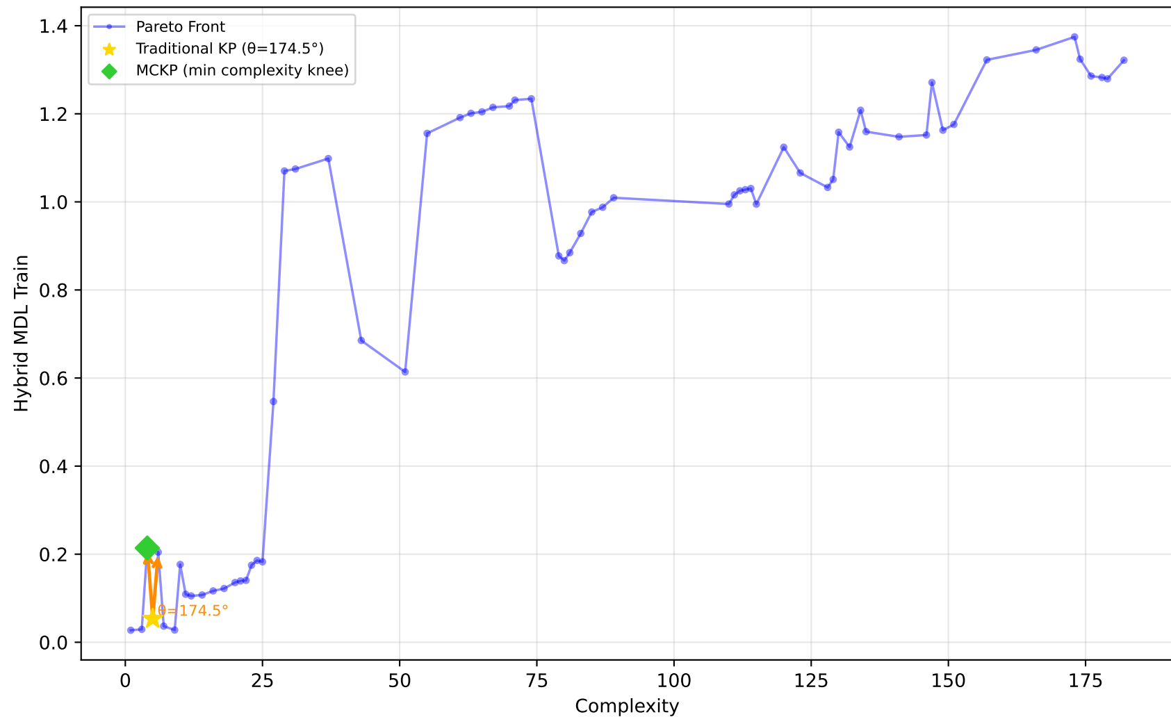
228_elusage - Run 28 - SVP - Hybrid MDL Train \lambda_1=0.00, \lambda_2=1.00, \lambda_3=0.00 | Difficulty: 0.53 | Method: mckp
