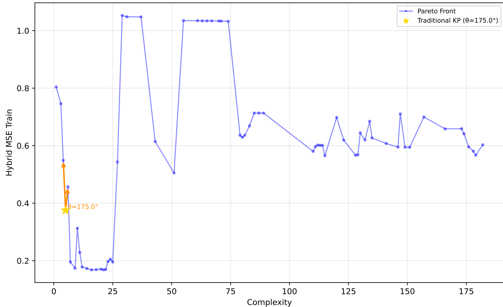
228_elusage - Run 28 - SVP - Hybrid MSE Train \lambda_1=0.00, \lambda_2=1.00, \lambda_3=0.00 | Difficulty: 0.53 | Method: mckp
