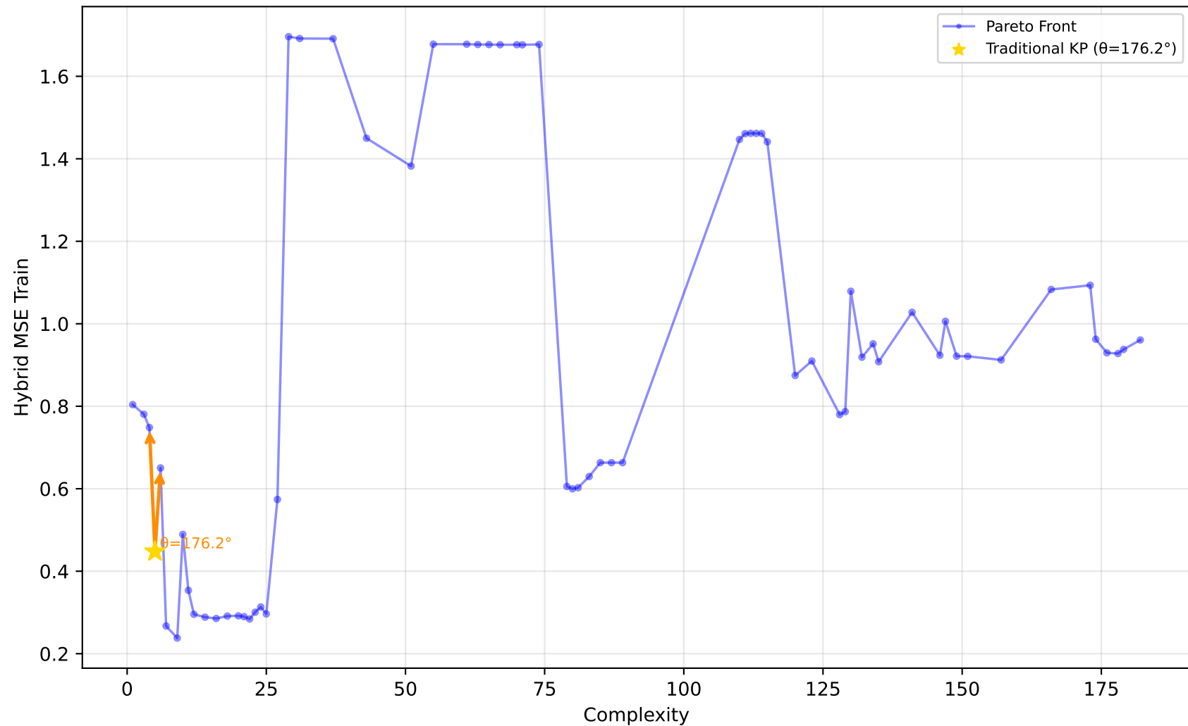
228_elusage - Run 28 - SVP - Hybrid MSE Train \lambda_1=0.60, \lambda_2=0.60, \lambda_3=1.00 | Difficulty: 0.53 | Method: mckp
