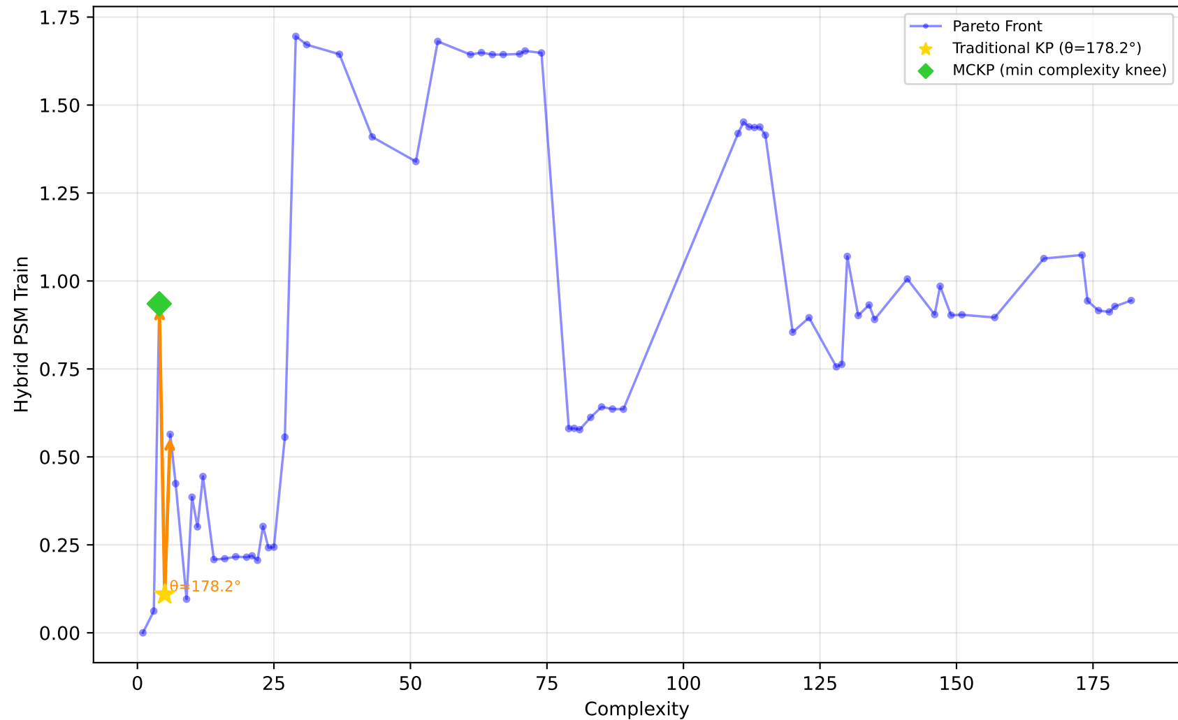
228_elusage - Run 28 - SVP - Hybrid PSM Train \lambda_1=0.60, \lambda_2=0.60, \lambda_3=1.00 | Difficulty: 0.53 | Method: mckp
