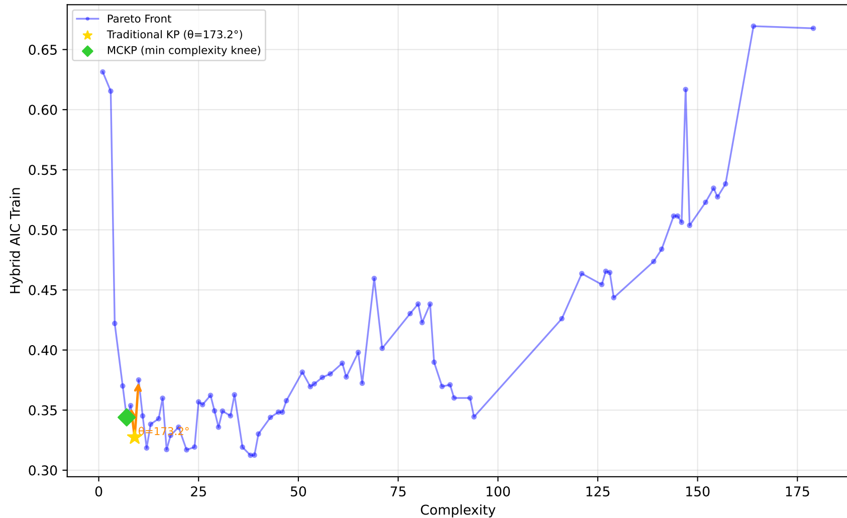
228_elusage - Run 29 - MVP - Hybrid AIC Train \lambda_1=0.00, \bar{\lambda}_2=0.00, \lambda_3=1.00 | Difficulty: 1.00 | Method: hmr
