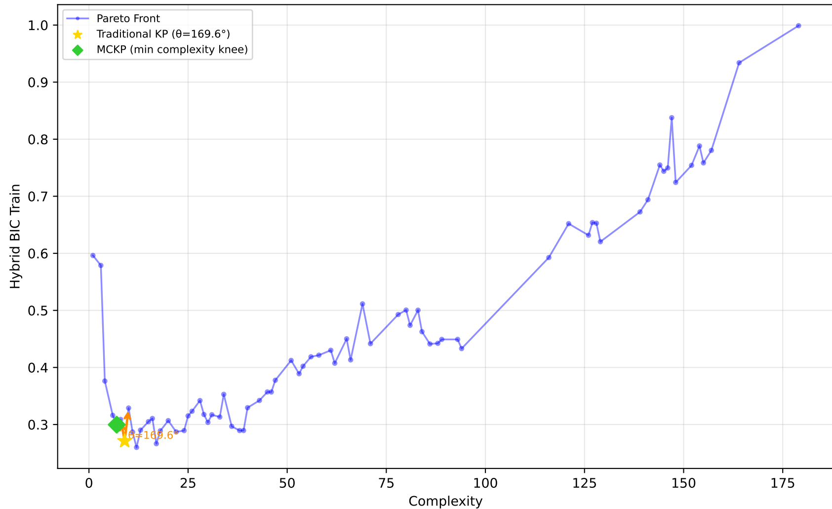
228_elusage - Run 29 - MVP - Hybrid BIC Train \lambda_1=0.00, \lambda_2=0.00, \lambda_3=1.00 | Difficulty: 1.00 | Method: hmr
