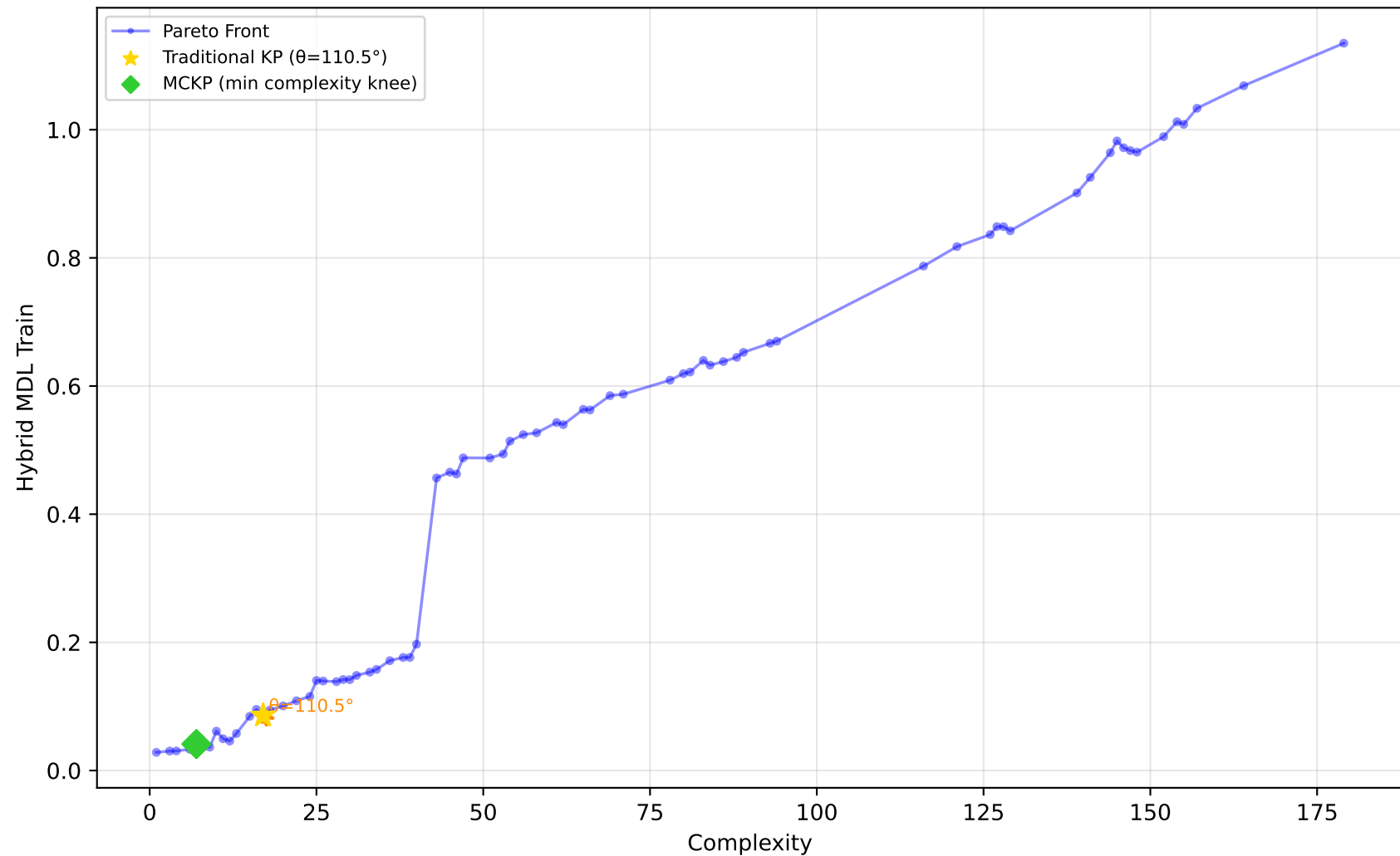
228_elusage - Run 29 - MVP - Hybrid MDL Train \lambda_1=0.00, \bar{\lambda}_2=0.30, \lambda_3=0.00 | Difficulty: 1.00 | Method: hmr
