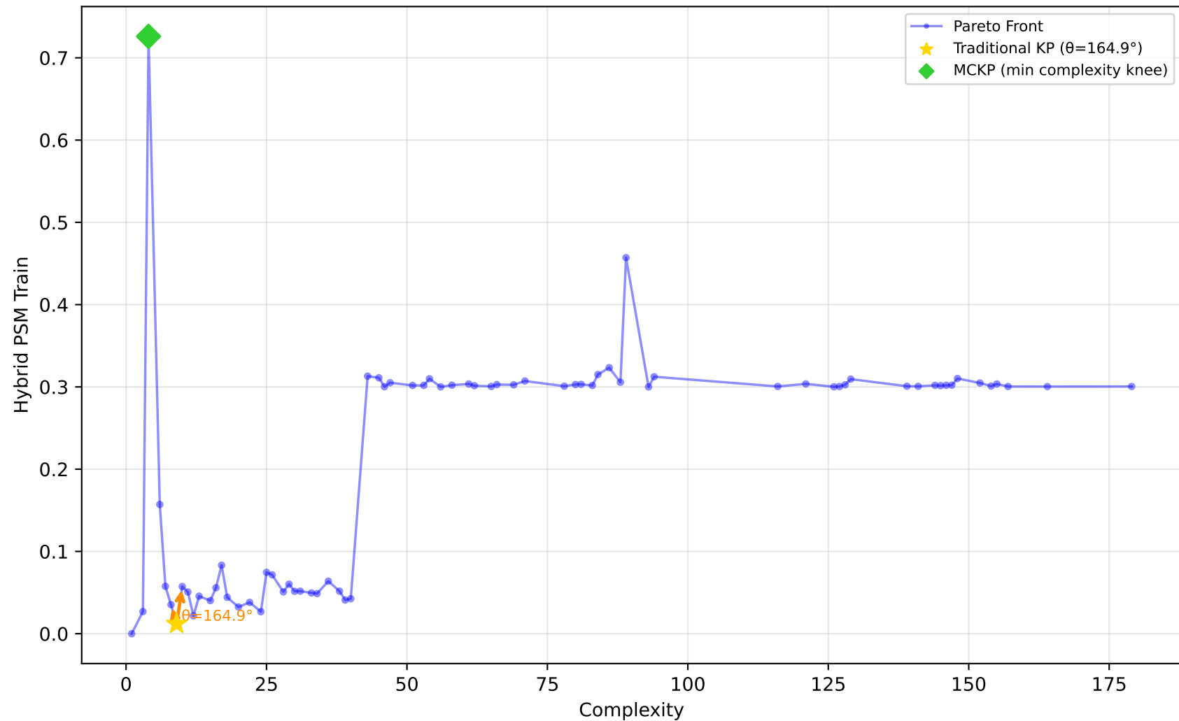
228_elusage - Run 29 - MVP - Hybrid PSM Train \lambda_1=0.00, \bar{\lambda}_2=0.30, \lambda_3=0.00 | Difficulty: 1.00 | Method: hmr
