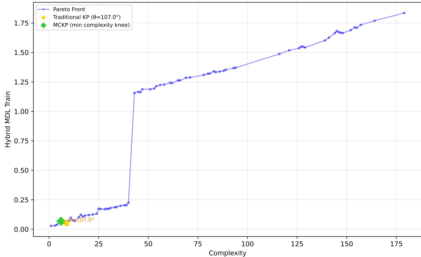
228_elusage - Run 29 - SVP - Hybrid MDL Train \lambda_1=0.00, \bar{\lambda}_2=1.00, \lambda_3=0.00 | Difficulty: 1.00 | Method: hmr
