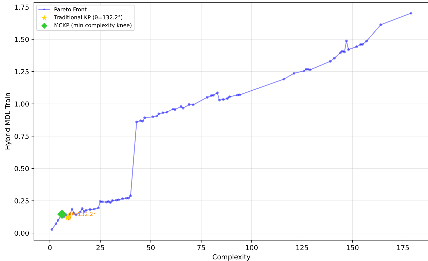
228_elusage - Run 29 - SVP - Hybrid MDL Train \lambda_1=0.60, \bar{\lambda}_2=0.60, \lambda_3=1.00 | Difficulty: 1.00 | Method: hmr
