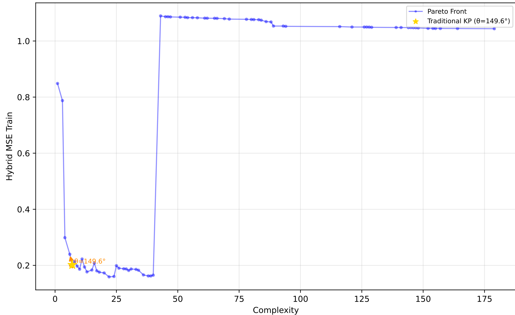
228_elusage - Run 29 - SVP - Hybrid MSE Train \lambda_1=0.00, \lambda_2=1.00, \lambda_3=0.00 | Difficulty: 1.00 | Method: hmr
