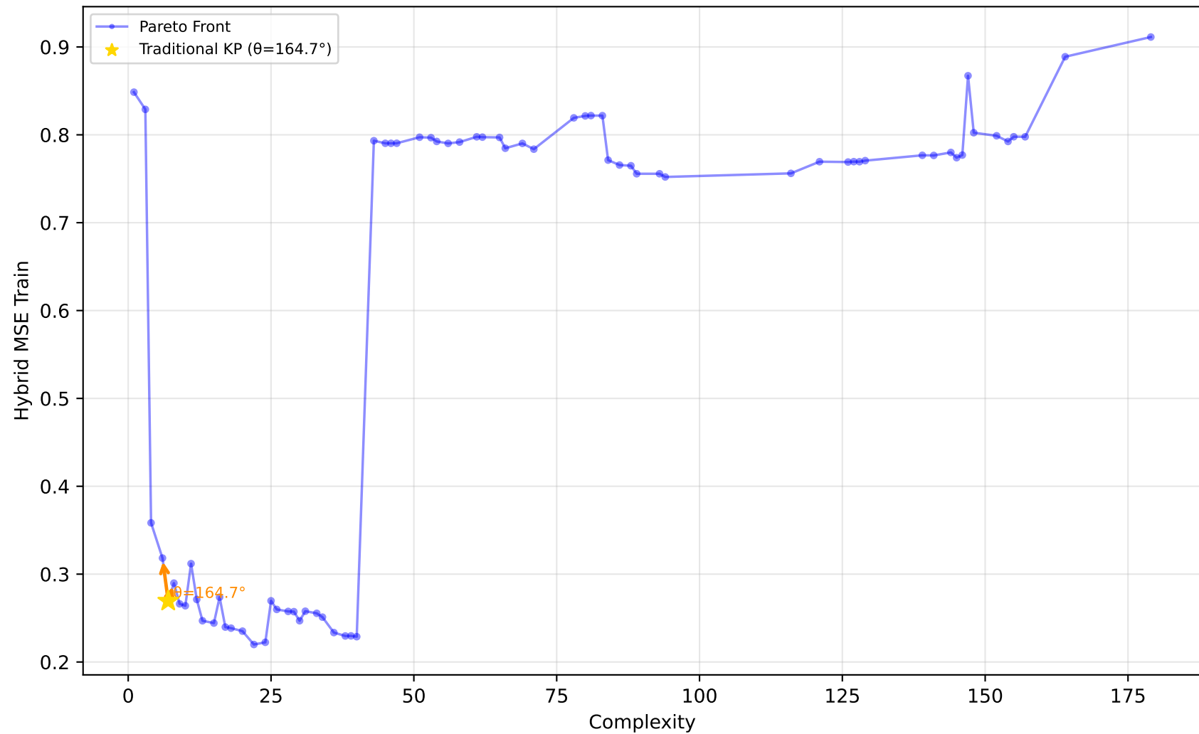
228_elusage - Run 29 - SVP - Hybrid MSE Train \lambda_1=0.60, \bar{\lambda}_2=0.60, \lambda_3=1.00 | Difficulty: 1.00 | Method: hmr
