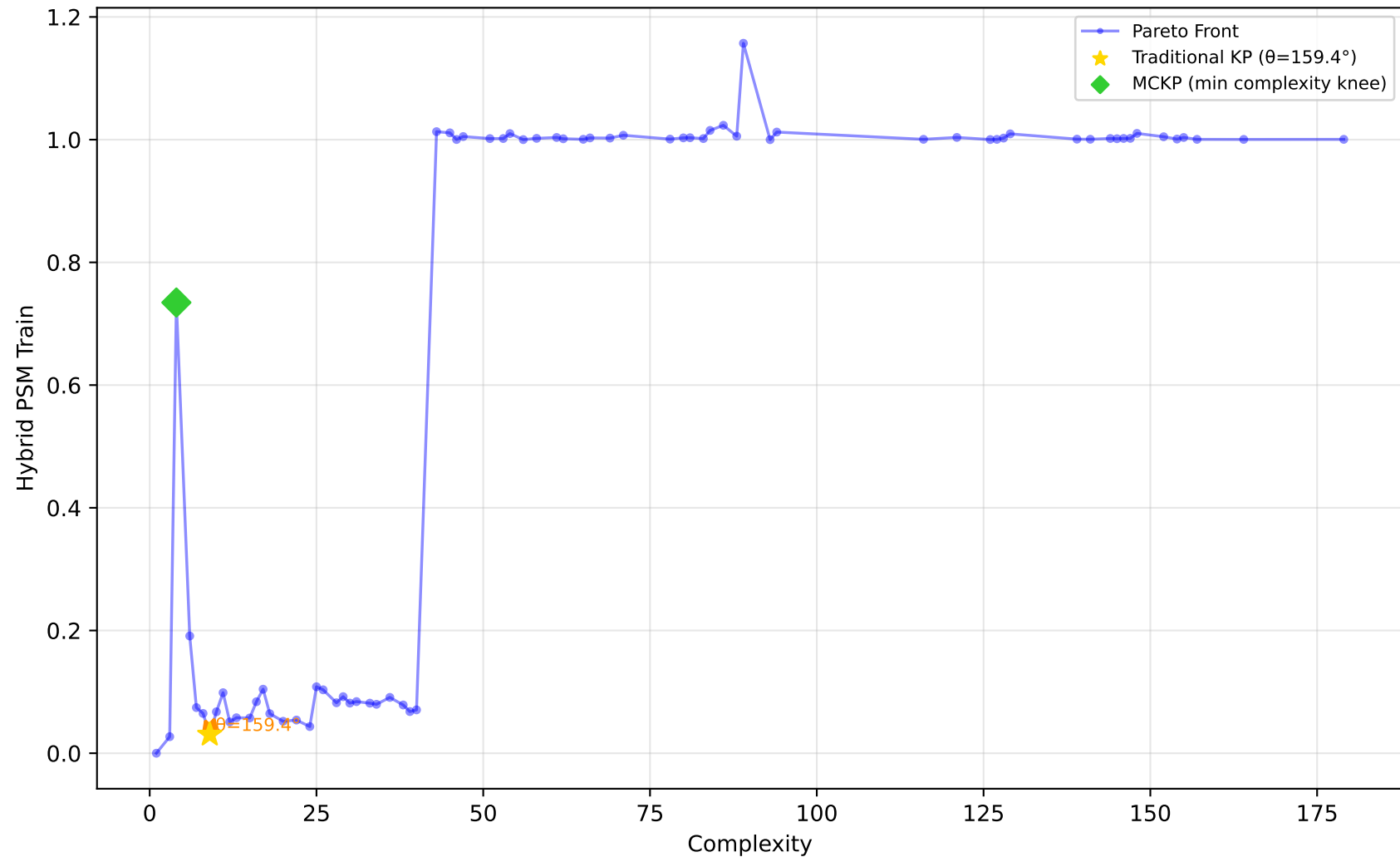
228_elusage - Run 29 - SVP - Hybrid PSM Train \lambda_1=0.00, \bar{\lambda}_2=1.00, \lambda_3=0.00 | Difficulty: 1.00 | Method: hmr
