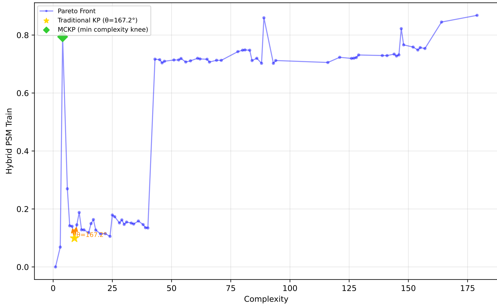
228_elusage - Run 29 - SVP - Hybrid PSM Train \lambda_1=0.60, \bar{\lambda}_2=0.60, \lambda_3=1.00 | Difficulty: 1.00 | Method: hmr
