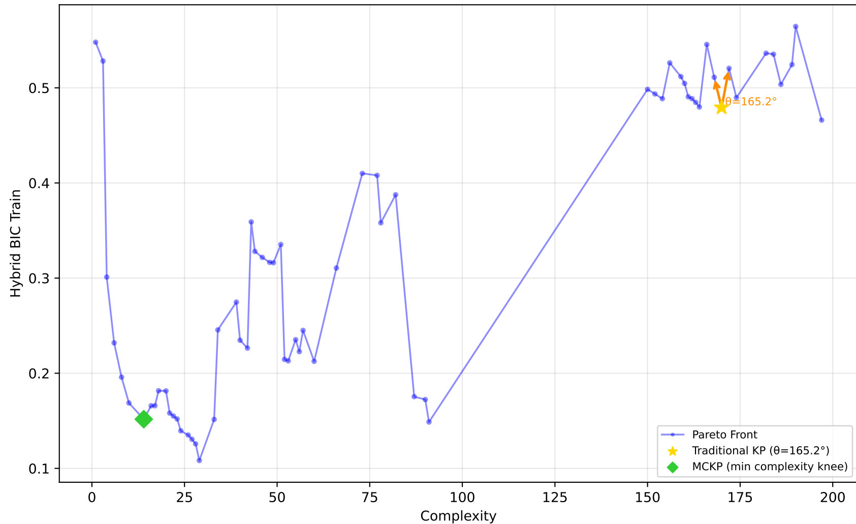
228_elusage - Run 2 - MVP - Hybrid BIC Train \lambda_1=0.00, \lambda_2=0.30, \lambda_3=0.00 | Difficulty: 0.62 | Method: hmr
