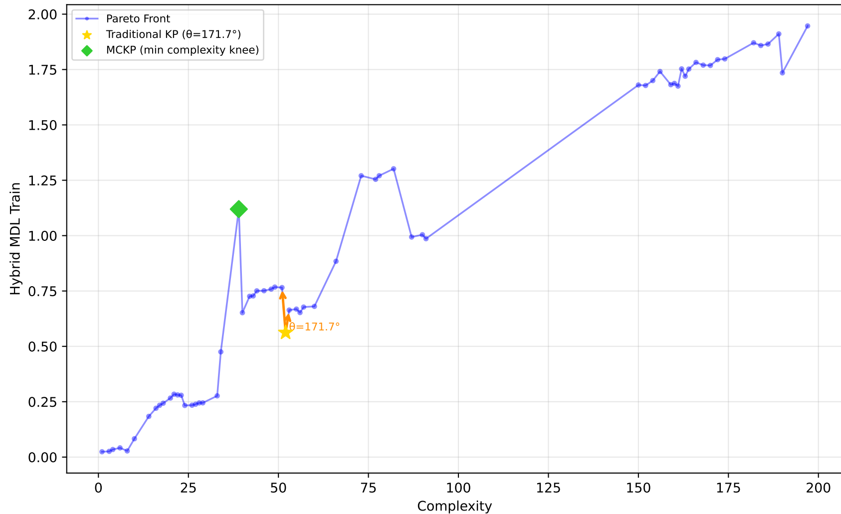
228_elusage - Run 2 - MVP - Hybrid MDL Train \lambda_1=0.00 , \lambda_2=0.00 , \lambda_3=1.00 | Difficulty: 0.62 | Method: hmr
