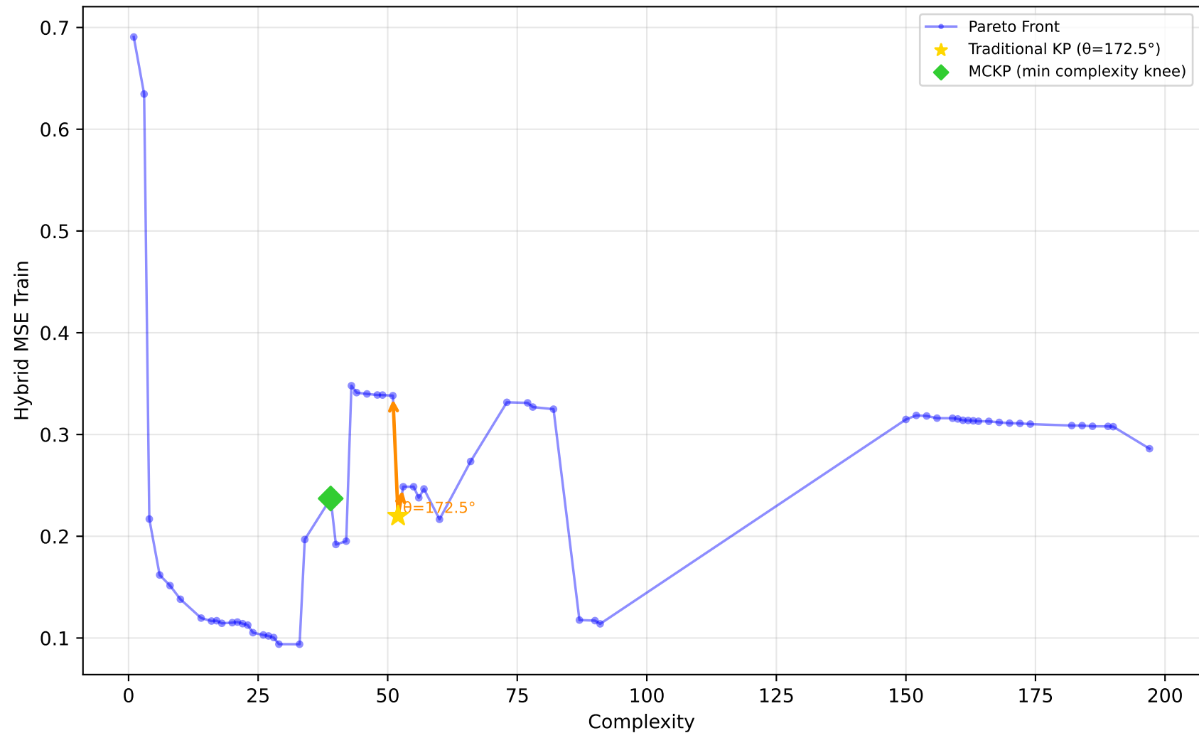
228_elusage - Run 2 - MVP - Hybrid MSE Train \lambda_1=0.00, \lambda_2=0.30, \lambda_3=0.00 | Difficulty: 0.62 | Method: hmr
