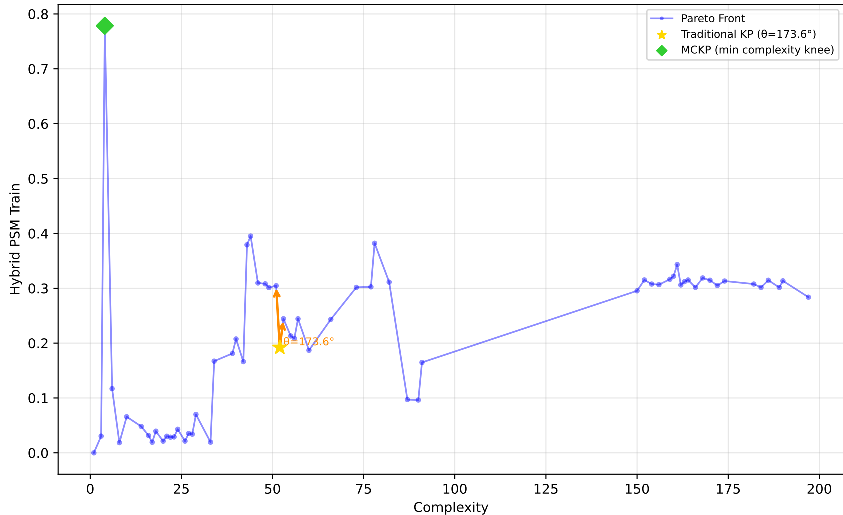
228_elusage - Run 2 - MVP - Hybrid PSM Train \lambda_1=0.00, \lambda_2=0.30, \lambda_3=0.00 | Difficulty: 0.62 | Method: hmr
