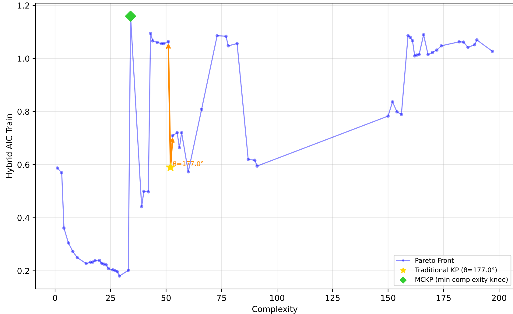
228_elusage - Run 2 - SVP - Hybrid AIC Train \lambda_1=0.00, \lambda_2=1.00, \lambda_3=0.00 | Difficulty: 0.62 | Method: hmr
