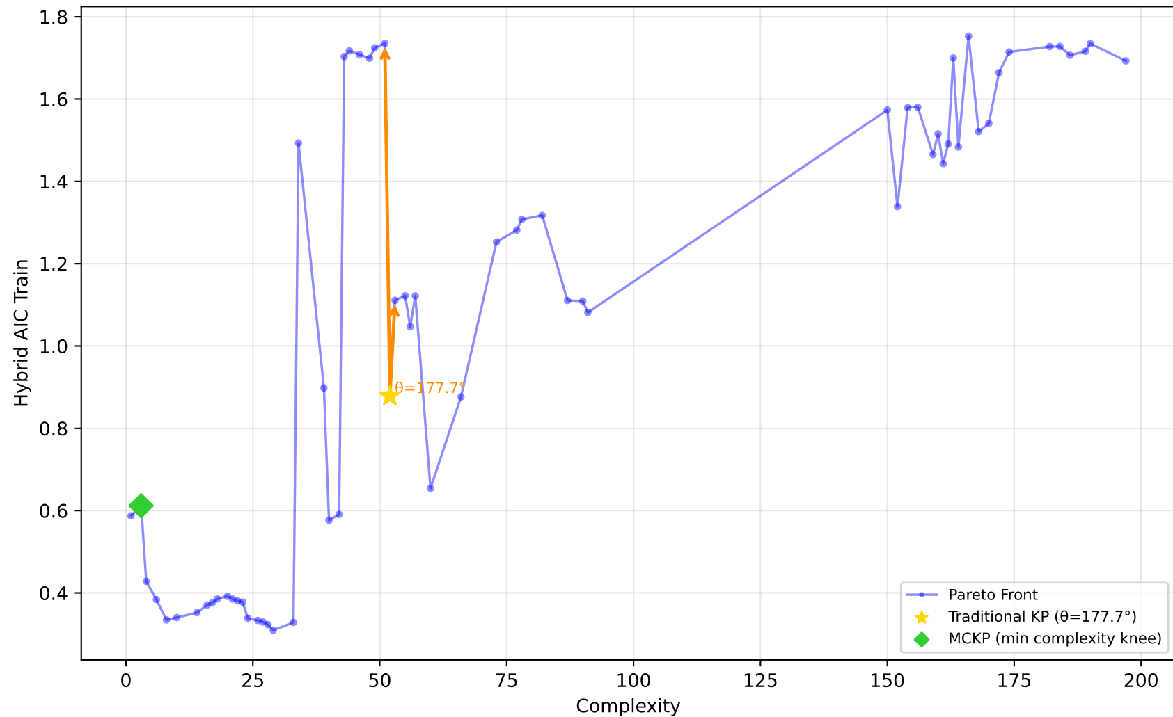
228_elusage - Run 2 - SVP - Hybrid AIC Train \lambda_1=0.60, \lambda_2=0.60, \lambda_3=1.00 | Difficulty: 0.62 | Method: hmr
