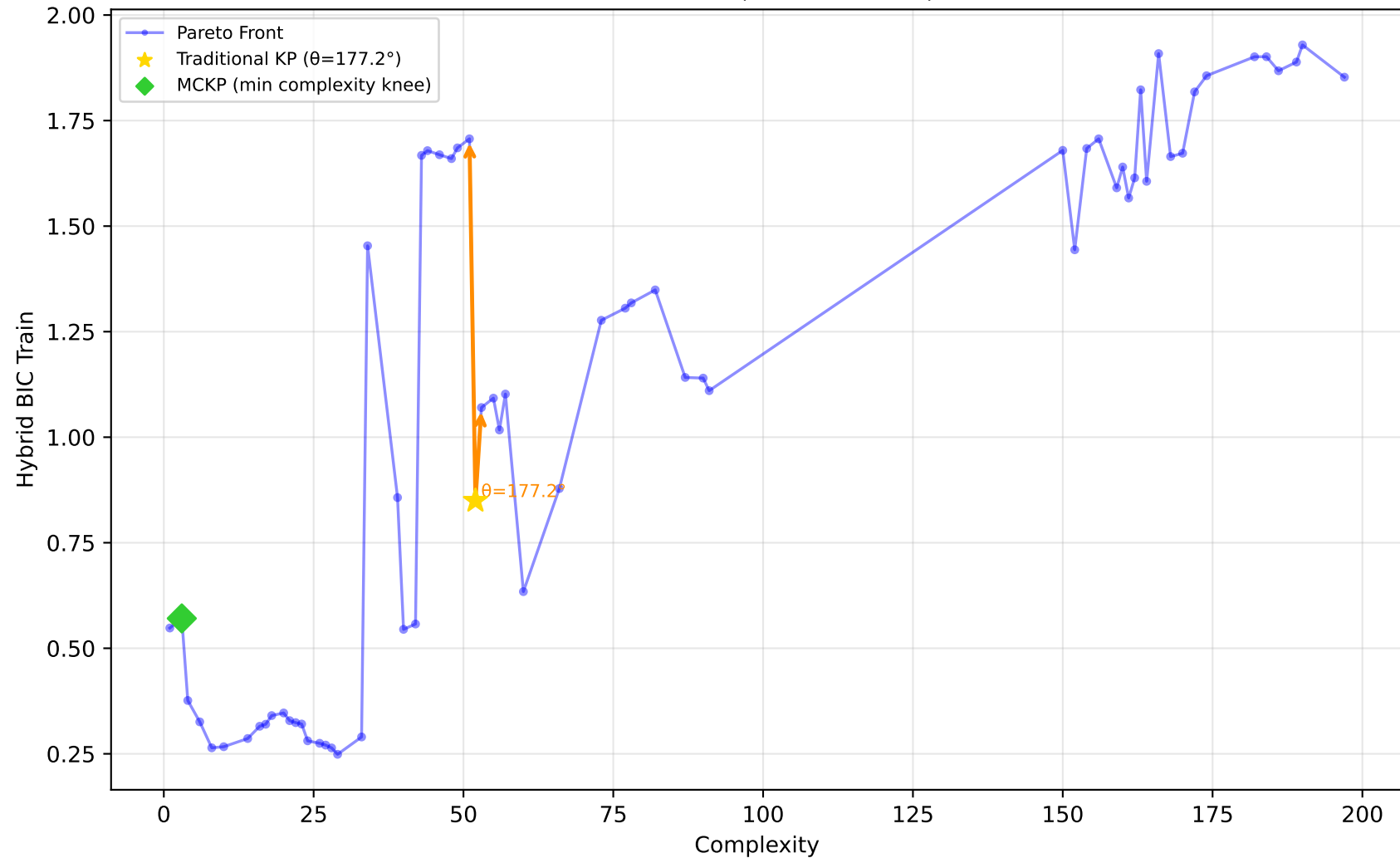
228_elusage - Run 2 - SVP - Hybrid BIC Train \lambda_1=0.60, \lambda_2=0.60, \lambda_3=1.00 | Difficulty: 0.62 | Method: hmr
