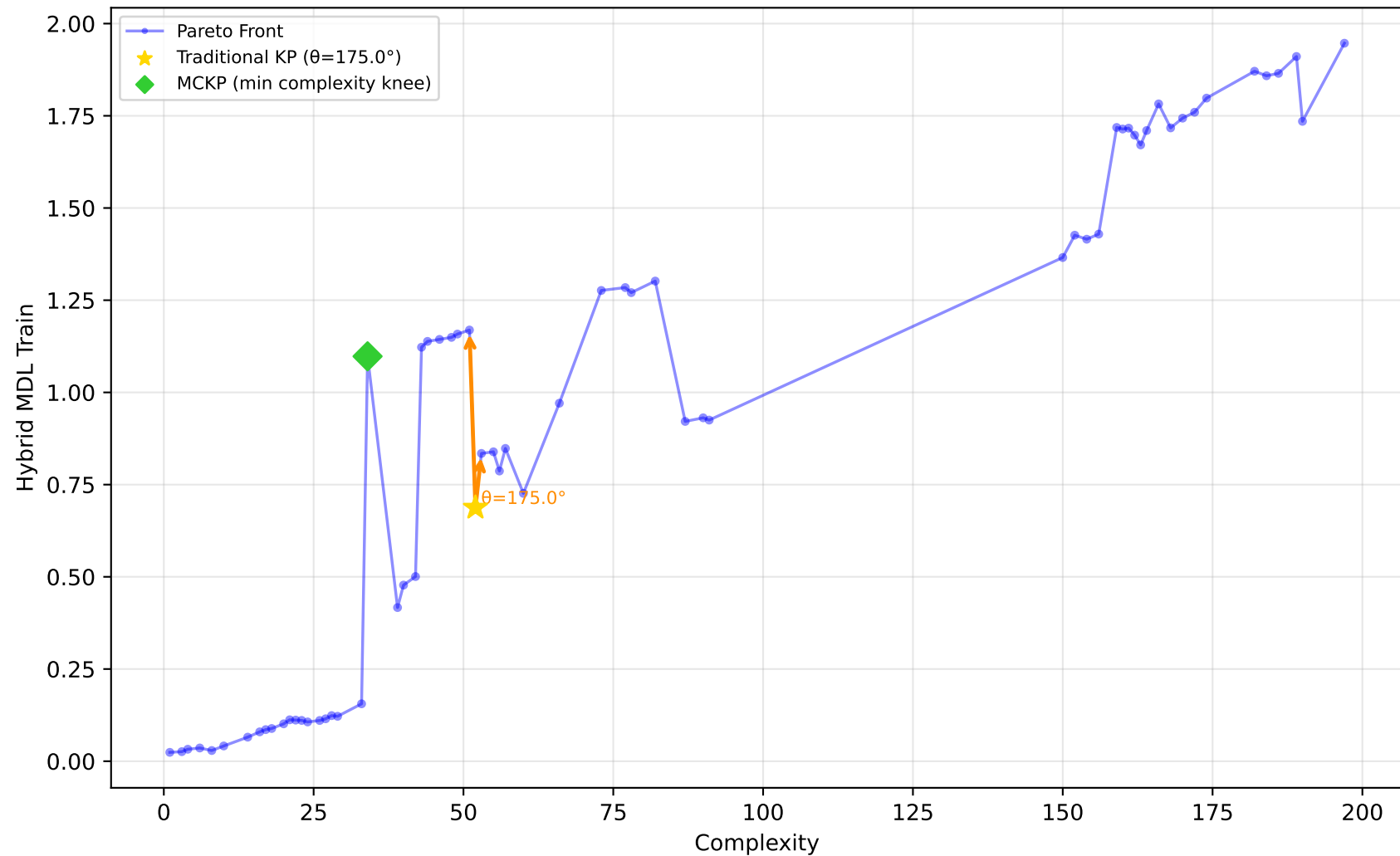
228_elusage - Run 2 - SVP - Hybrid MDL Train \lambda_1=0.00 , \lambda_2=1.00 , \lambda_3=0.00 | Difficulty: 0.62 | Method: hmr
