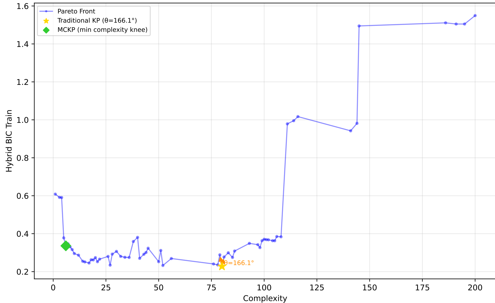
228_elusage - Run 30 - MVP - Hybrid BIC Train \lambda_1=0.00, \lambda_2=0.00, \lambda_3=1.00 | Difficulty: 0.45 | Method: mckp
