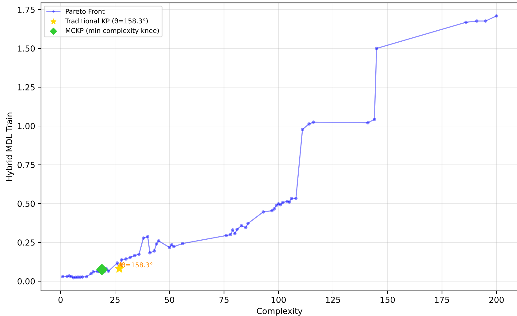
228_elusage - Run 30 - MVP - Hybrid MDL Train \lambda_1=0.00, \lambda_2=0.00, \lambda_3=1.00 | Difficulty: 0.45 | Method: mckp
