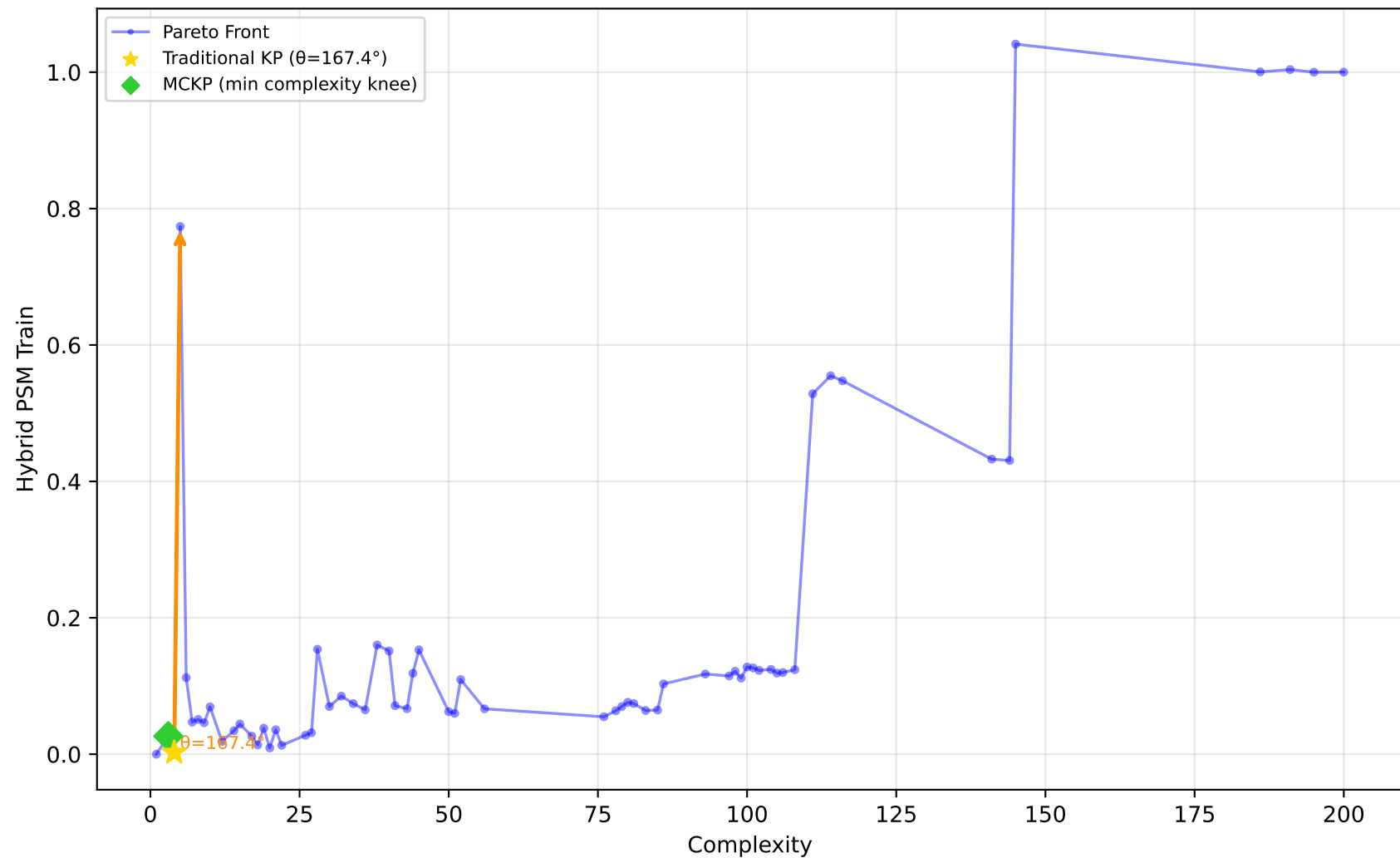
228_elusage - Run 30 - MVP - Hybrid PSM Train \lambda_1=0.00, \lambda_2=0.00, \lambda_3=1.00 | Difficulty: 0.45 | Method: mckp
